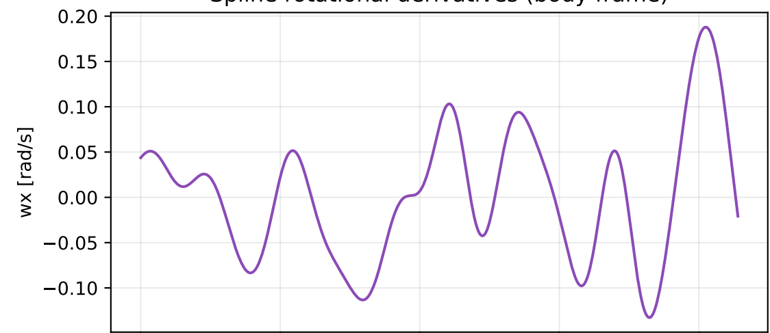
Spline rotational derivatives (body frame)
