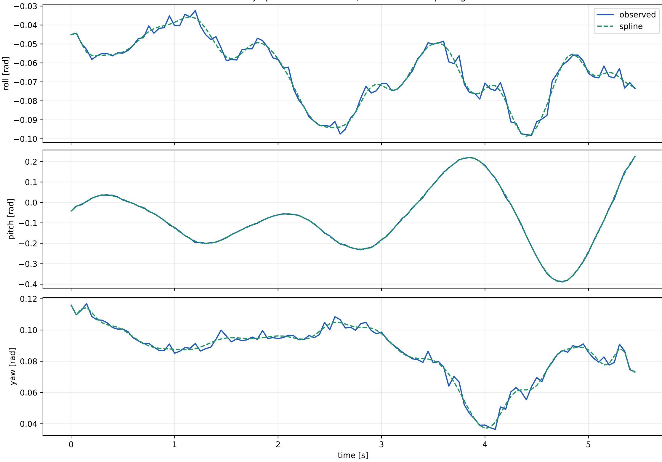
Pose-only spline orientation fit; selected knot spacing=0.2s
