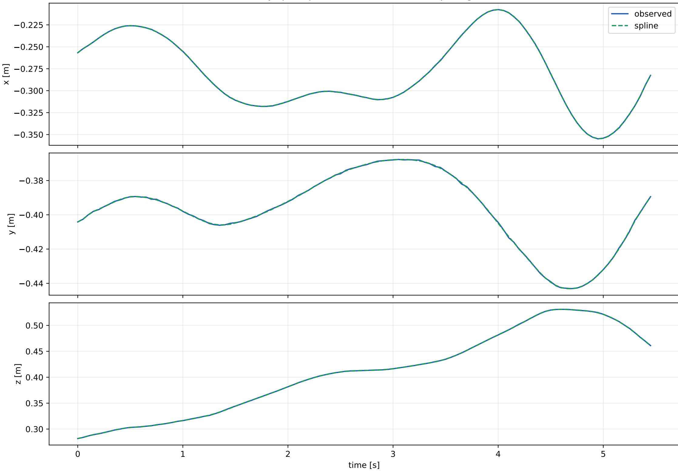
Pose-only spline position fit; selected knot spacing=0.2s
