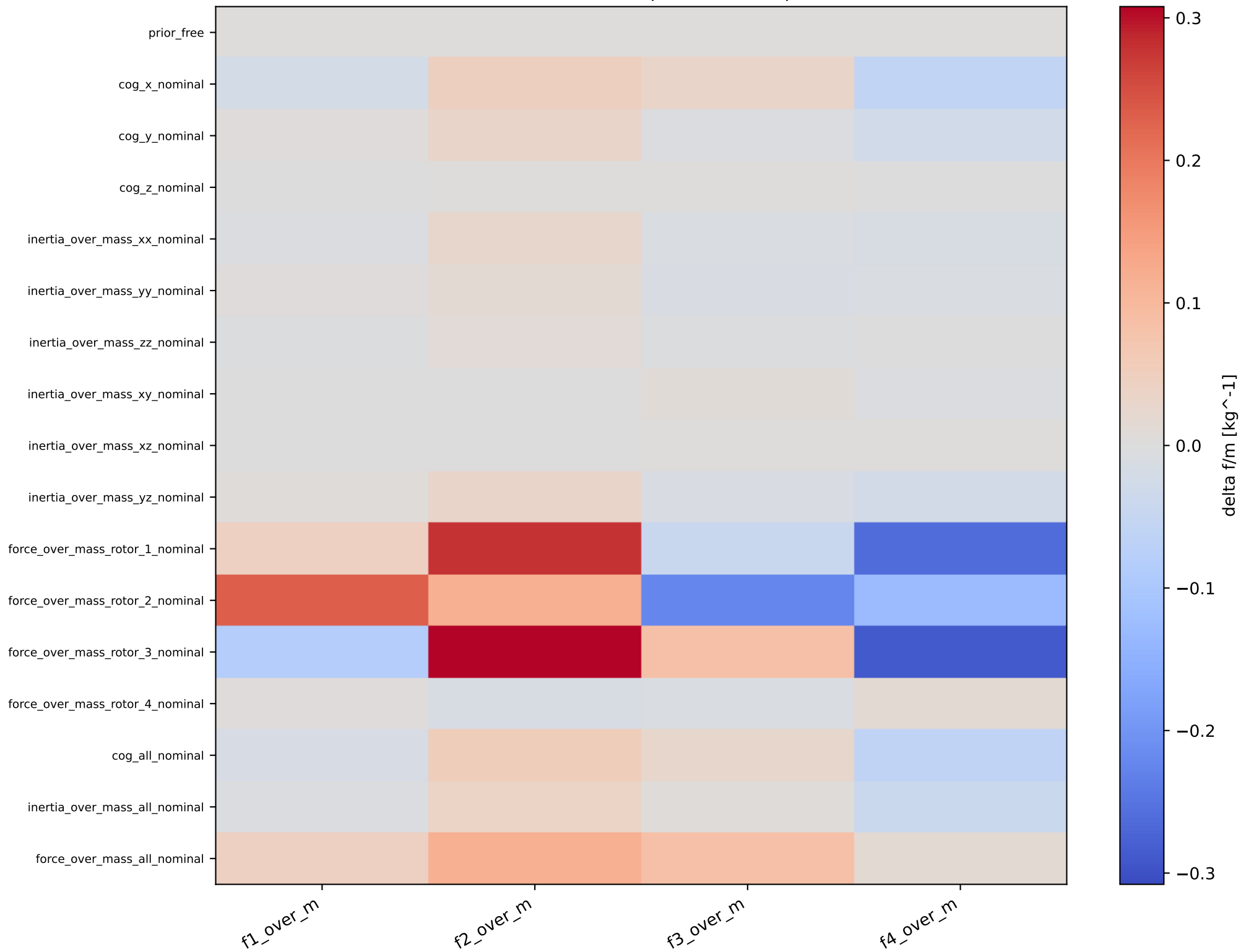
Force-over-mass compensation response
