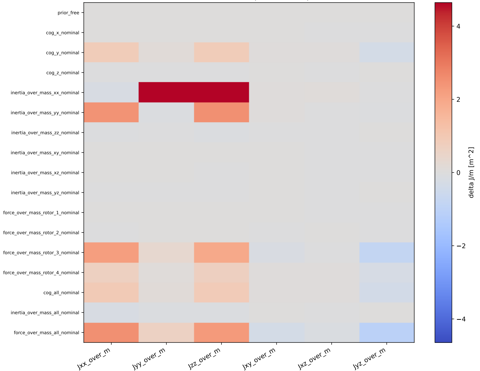
Inertia-over-mass compensation response
