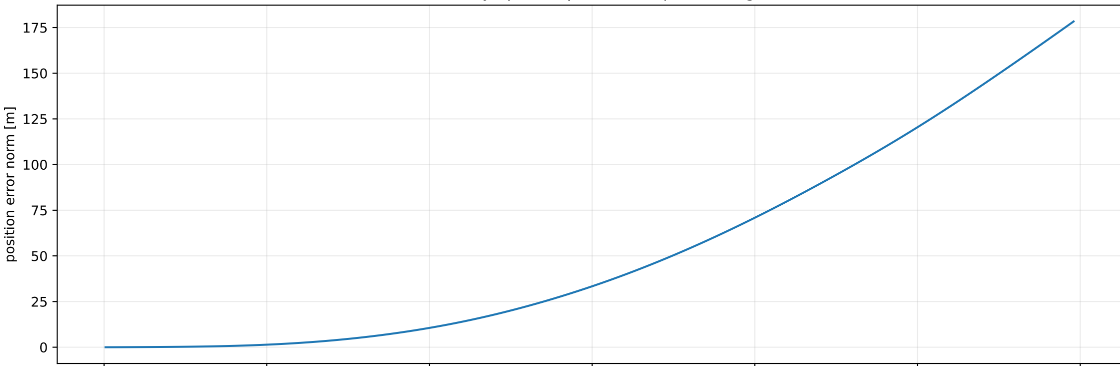
Parameter-only open-loop rollout (separate diagnostic)
