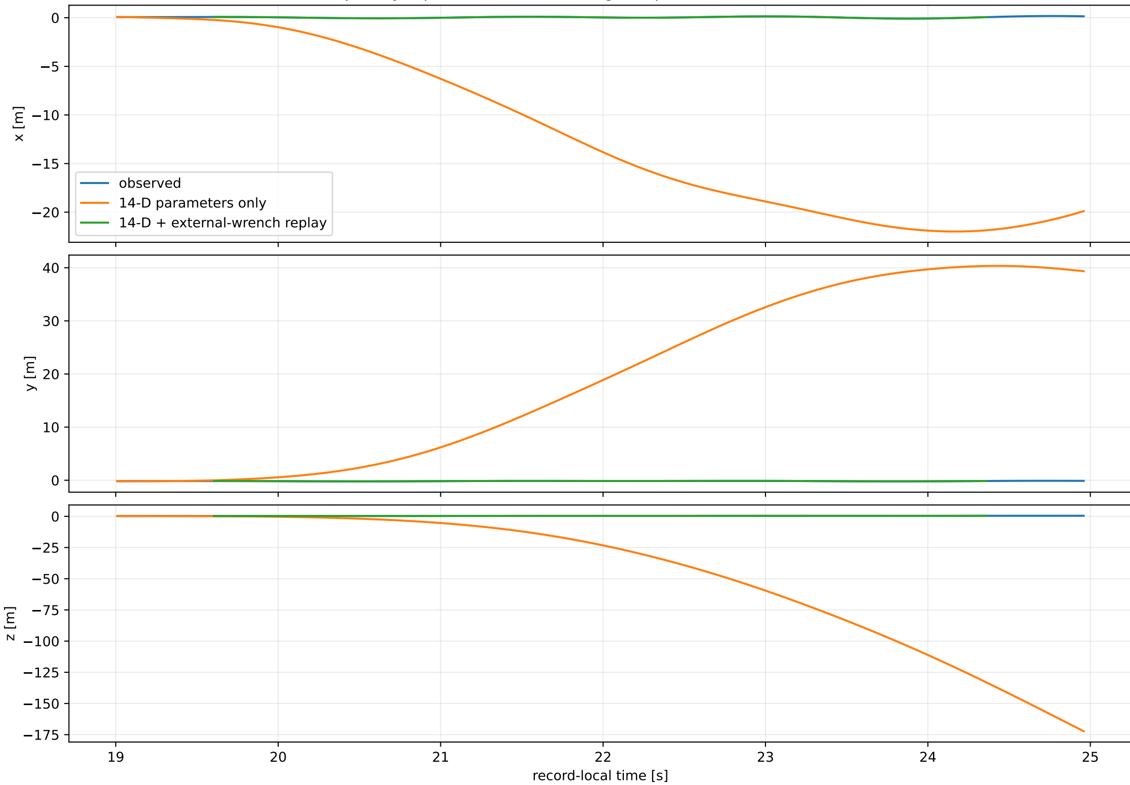
Trajectory reproduction after adding independent rotor effectiveness
