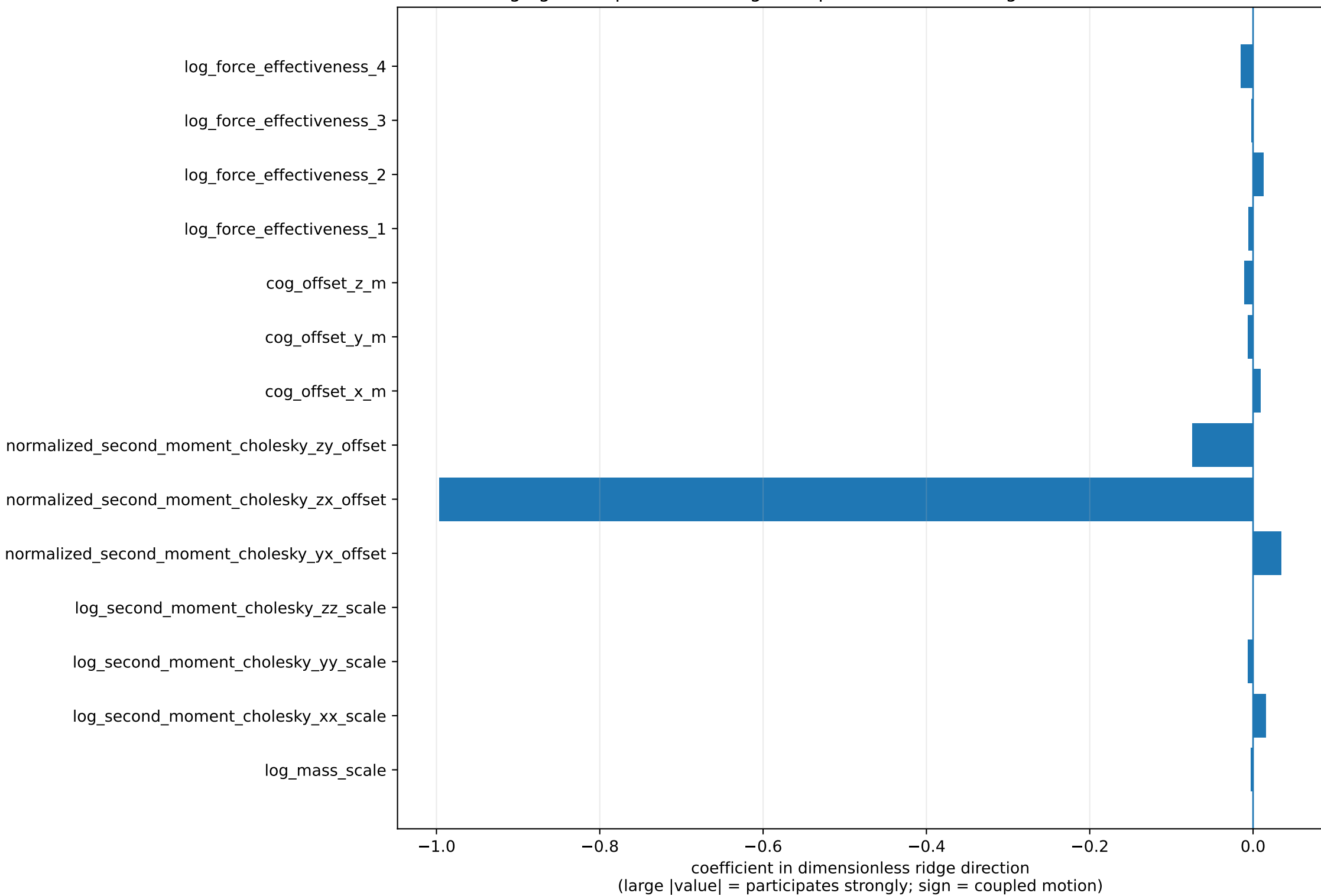
Ridge direction 2: relative information = 1.516 \times 10^{-5} Changing these parameters together produces little change in the wrench likelihood
