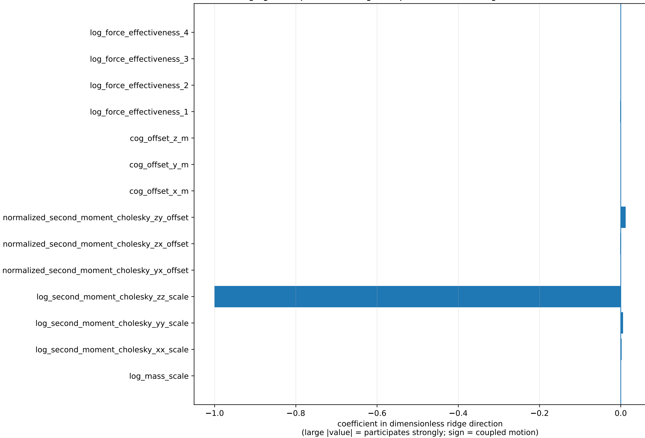
Ridge direction 1: relative information = 8.210\text{e-}09 Changing these parameters together produces little change in the wrench likelihood
