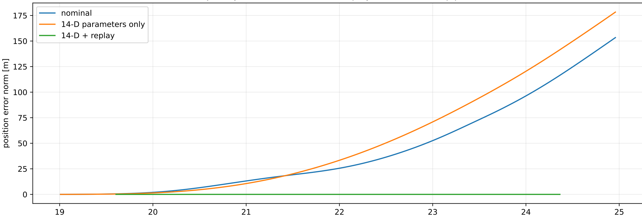
Trajectory error: lower is better; replay verifies the full pipeline
