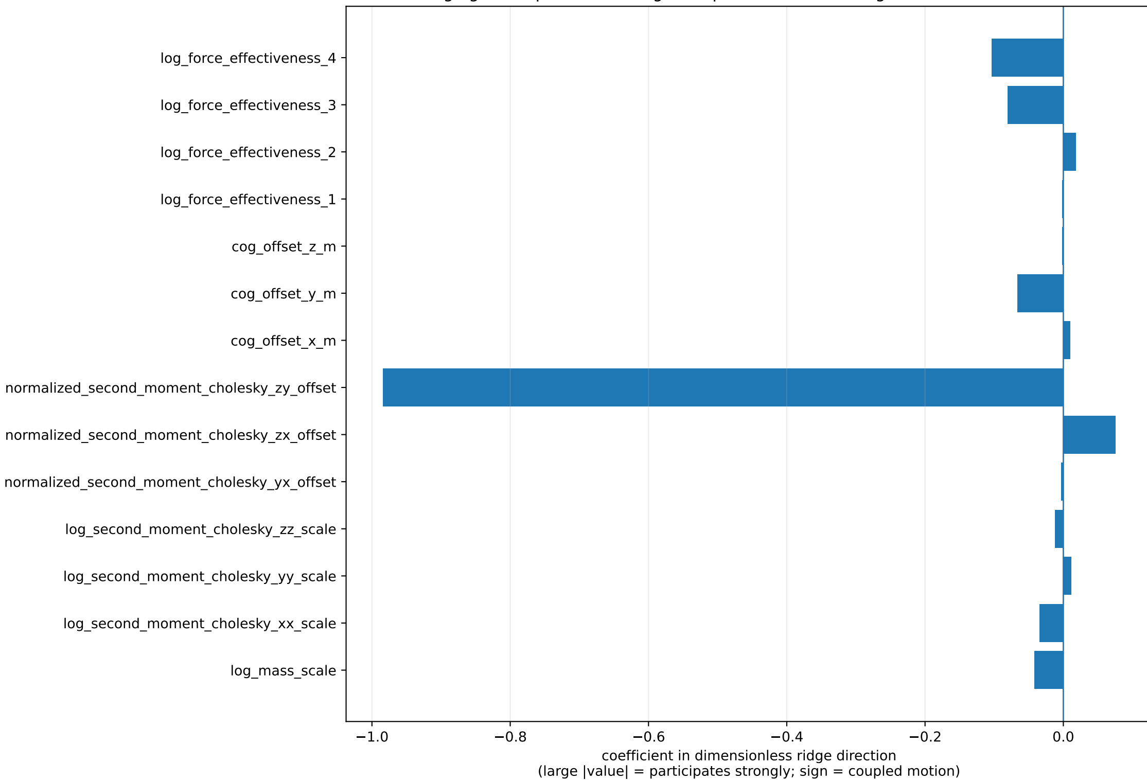
Ridge direction 3: relative information = 3.400\text{e-}05 Changing these parameters together produces little change in the wrench likelihood
