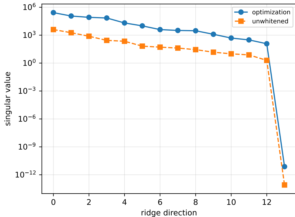
cov_full_no_R_uncertainty_in_s: ridge spectrum (rank 13, nullity 1, ||jv||=1.75e-11)
