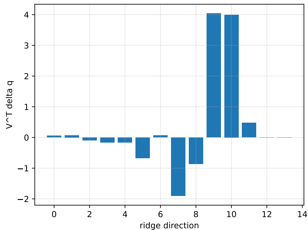
cov_full_no_R_uncertainty_in_s: ridge spectrum (rank 13, nullity 1, ||jv||=1.75e-11)
