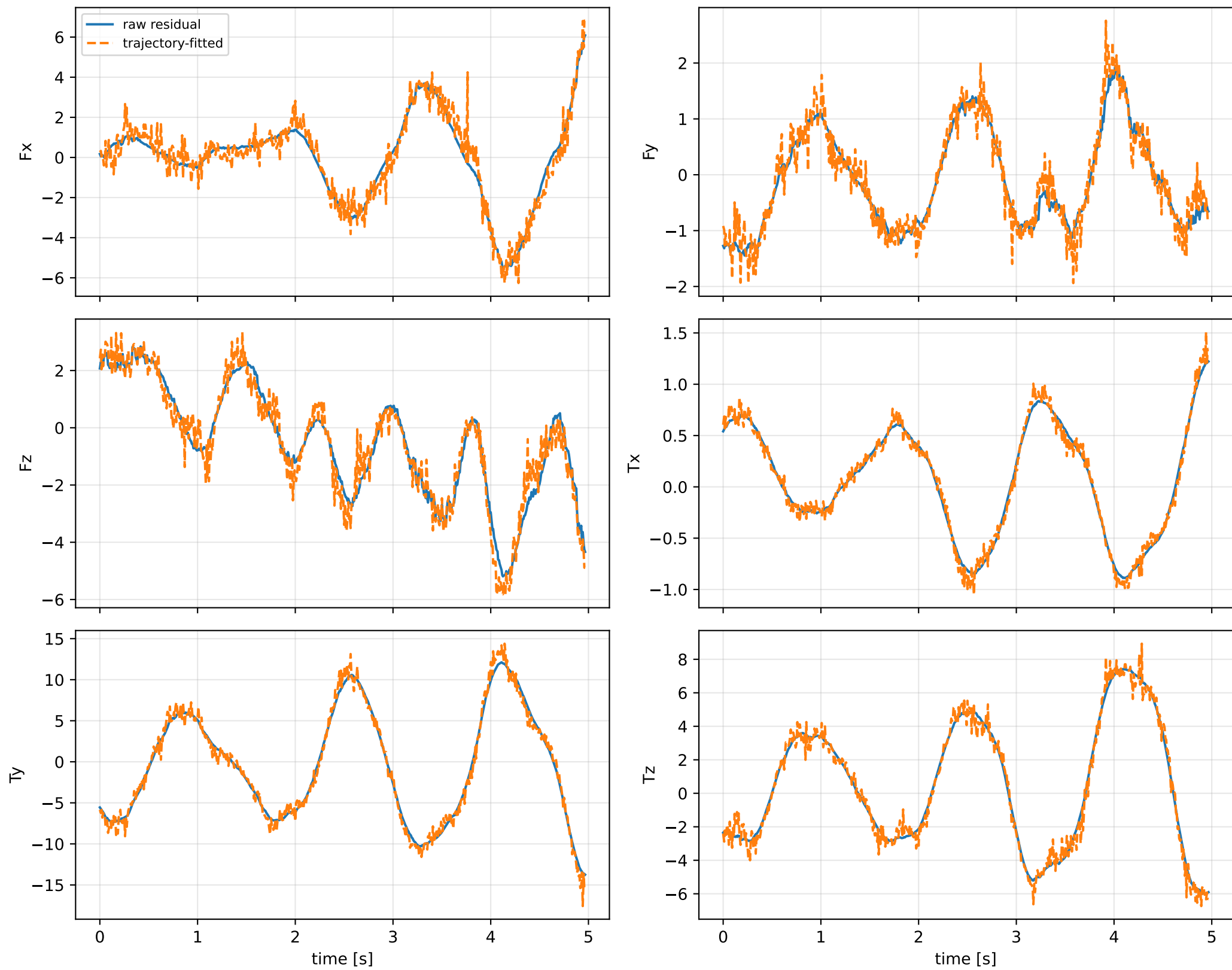
cov_full_no_position_rotation_cross: wrench / closure (force max 2.09\text{e-}14 , torque max 5.33\text{e-}15 )
