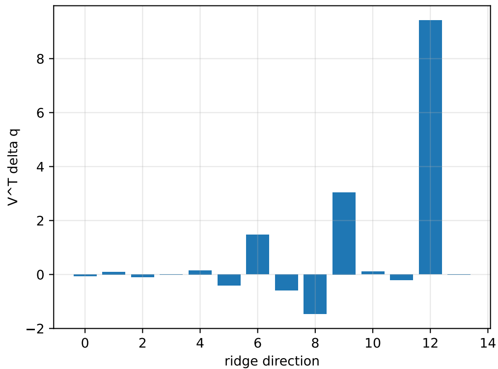
cov_full_no_position_rotation_cross: ridge spectrum (rank 13, nullity 1, ||v||=1.22e-11)
