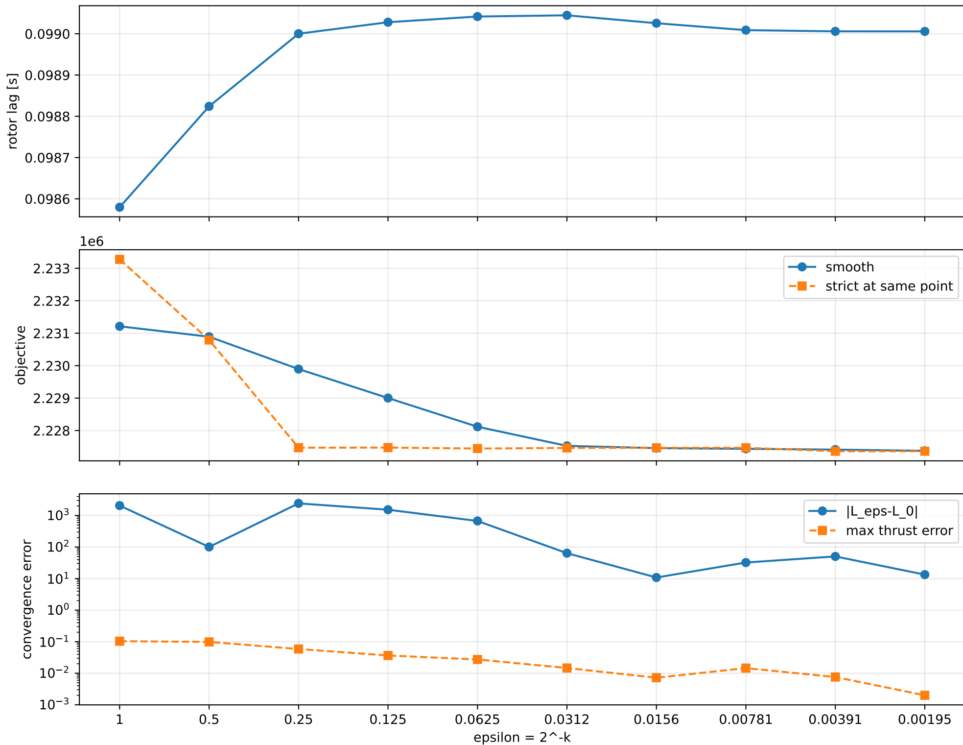
cov_full_no_position_rotation_cross: smooth-to-strict continuation
