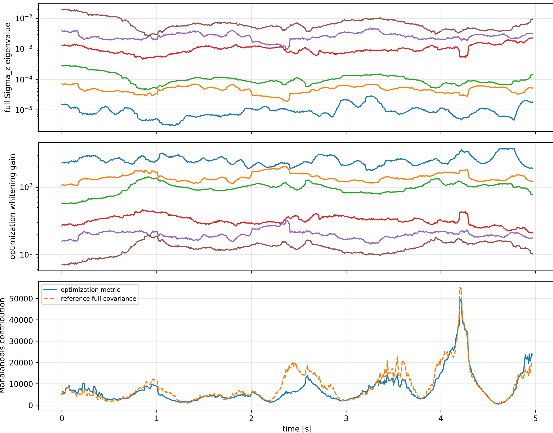
cov_full_no_position_rotation_cross: optimization vs reference covariance
