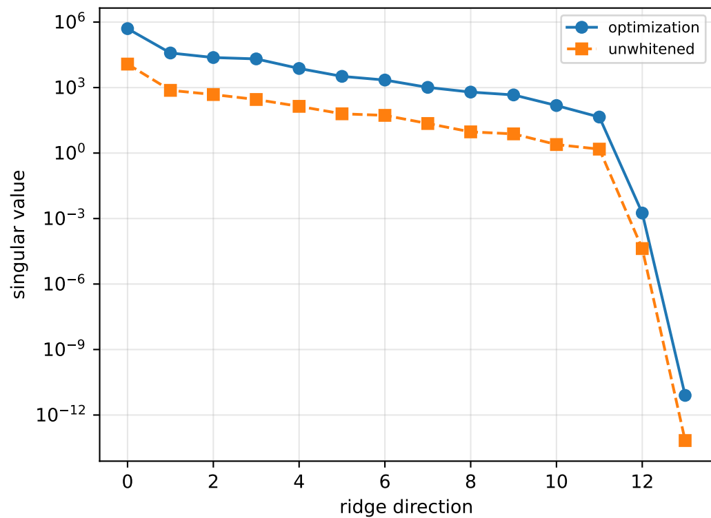
cov_full_no_position_rotation_cross: ridge spectrum (rank 13, nullity 1, ||v||=1.22e-11)
