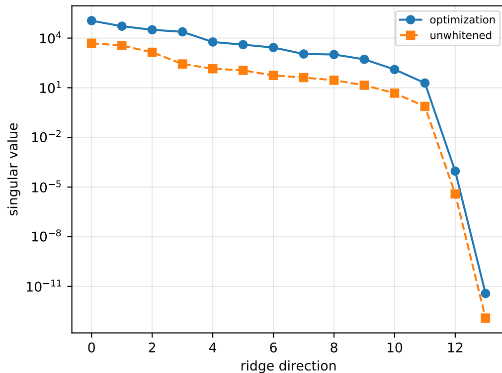
cov_global_full: ridge spectrum (rank 13, nullity 1, ||jv||=6.43e-12)
