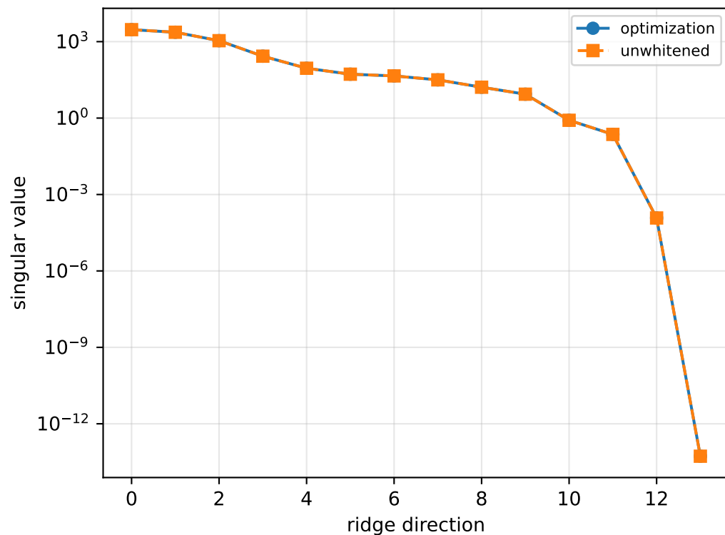
kkt_scale_positive: ridge spectrum (rank 13, nullity 1, ||Jv||=1.25e-13)
