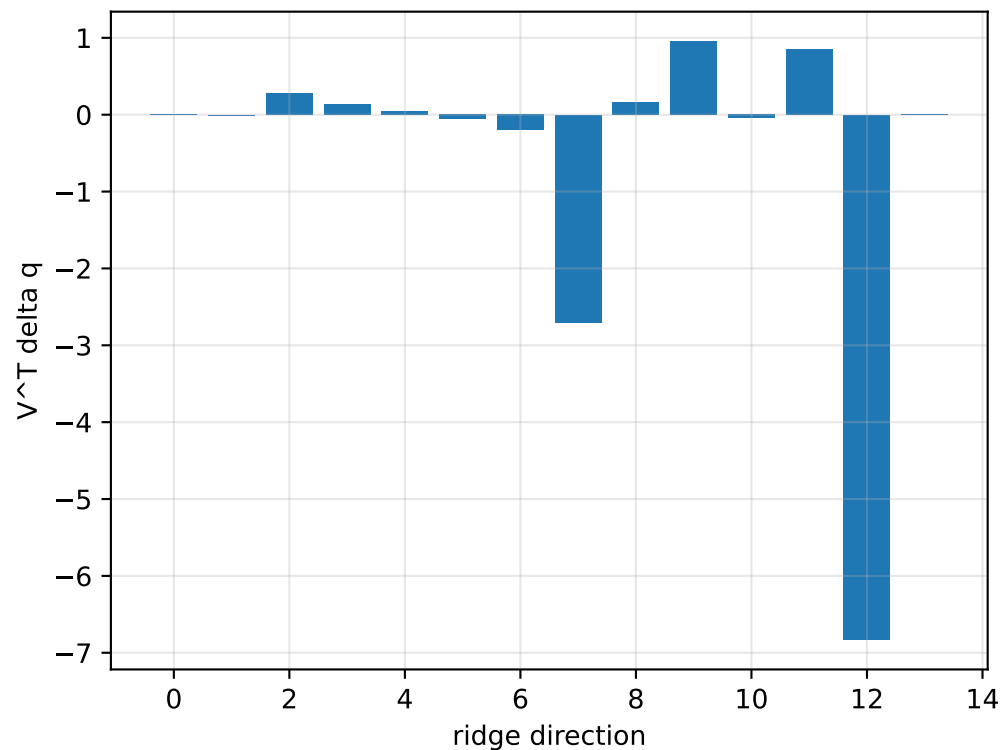
kkt_scale_positive: ridge spectrum (rank 13, nullity 1, ||Jv||=1.25e-13)
