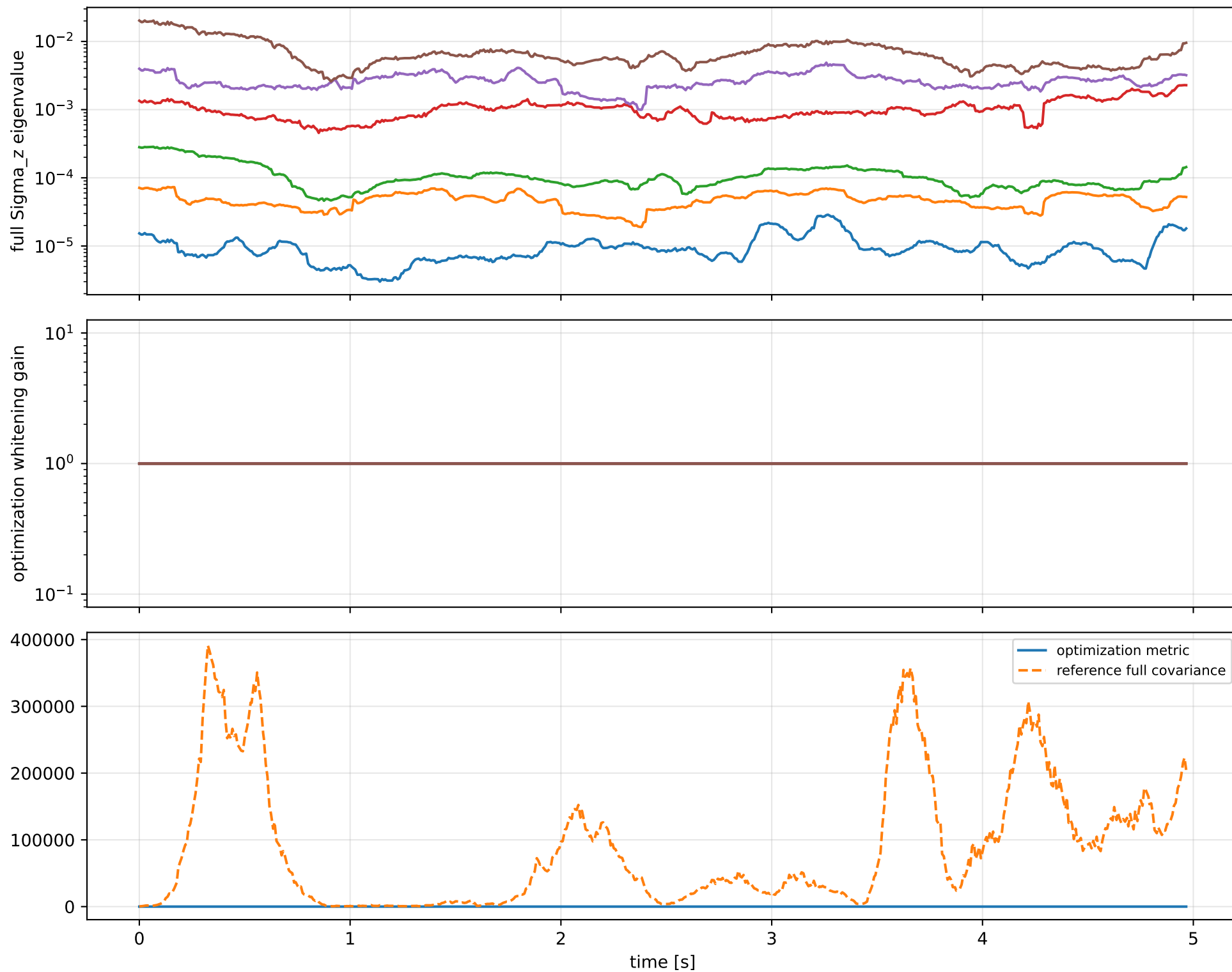
lag_fixed_one_period: optimization vs reference covariance
