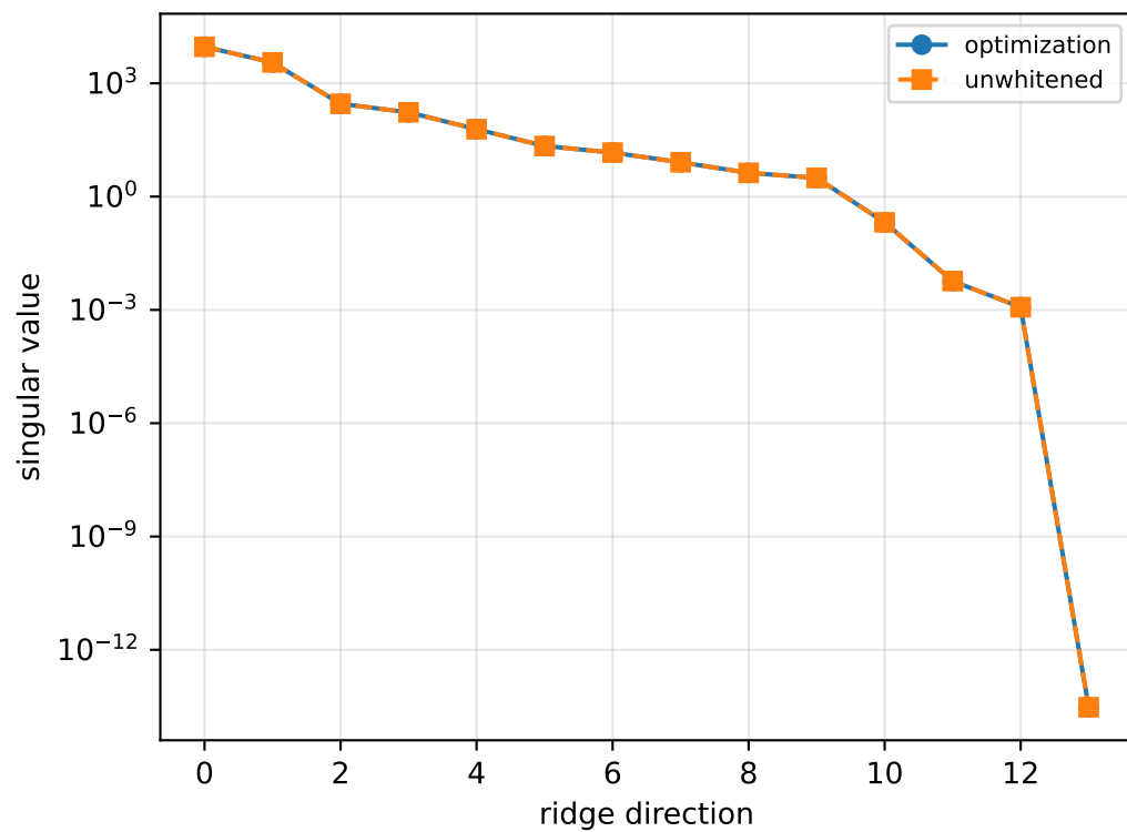
lag_fixed_one_period: ridge spectrum (rank 13, nullity 1, ||jv||=1.73e-13 )
