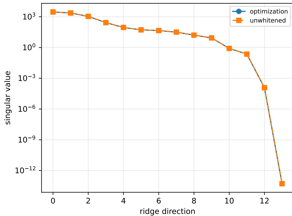
lag_pow2_depth_12: ridge spectrum (rank 13, nullity 1, \|Jv\|=1.03e-13 )
