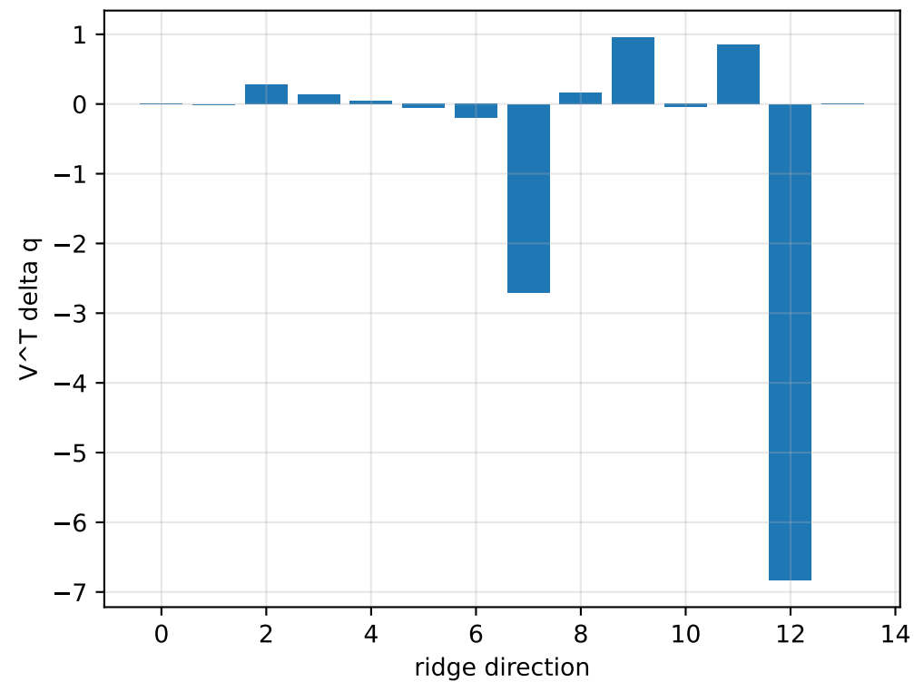
lag_pow2_depth_12: ridge spectrum (rank 13, nullity 1, \|Jv\|=1.03e-13 )
