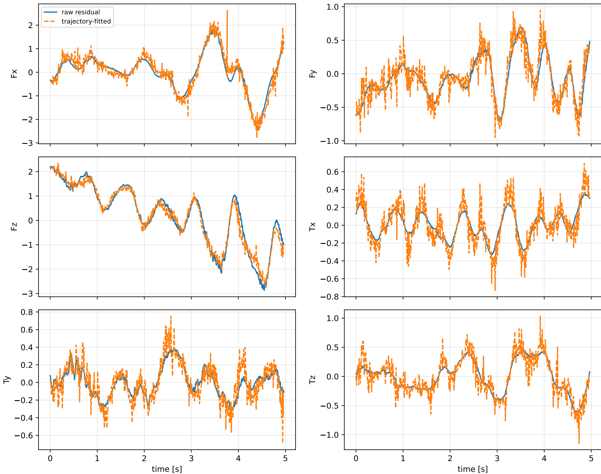
lag_pow2_depth_12: wrench / closure (force max 1.04\text{e-}14 , torque max 1.11\text{e-}15 )
