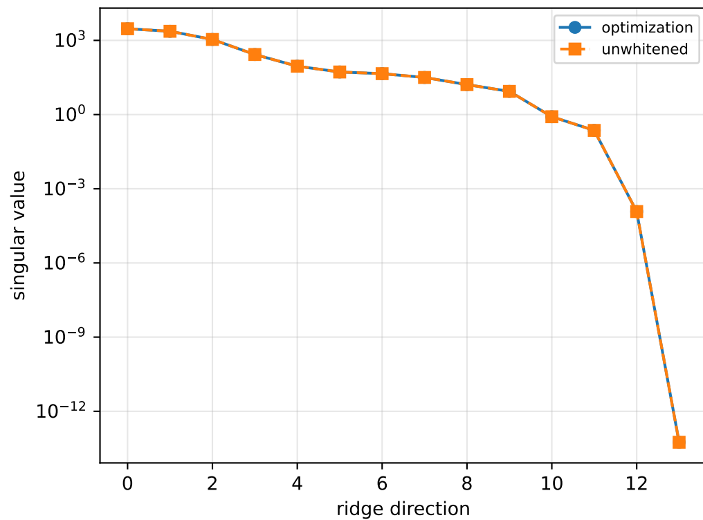
lag_pow2_depth_6: ridge spectrum (rank 13, nullity 1, ||Jv||=1.5e-13)
