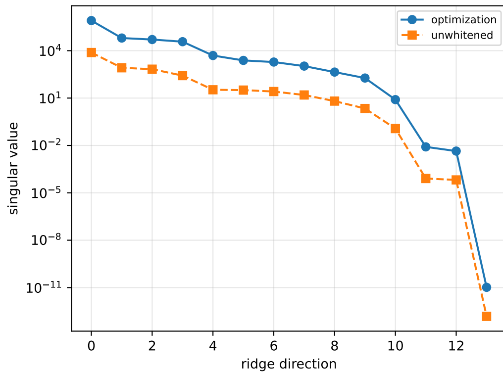
cov_block_s_alpha: ridge spectrum (rank 13, nullity 1, ||v||=2.25e-11)
