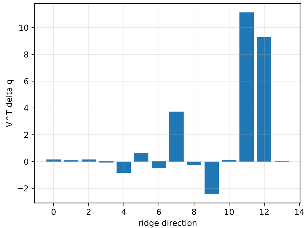
cov_block_s_alpha: ridge spectrum (rank 13, nullity 1, ||v||=2.25e-11)
