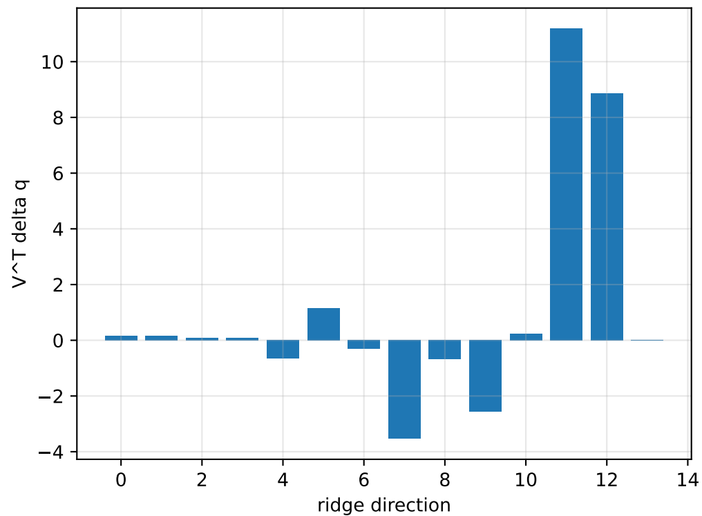
cov_full_no_position_rotation_cross: ridge spectrum (rank 13, nullity 1, ||Jv||=2.06e-11)
