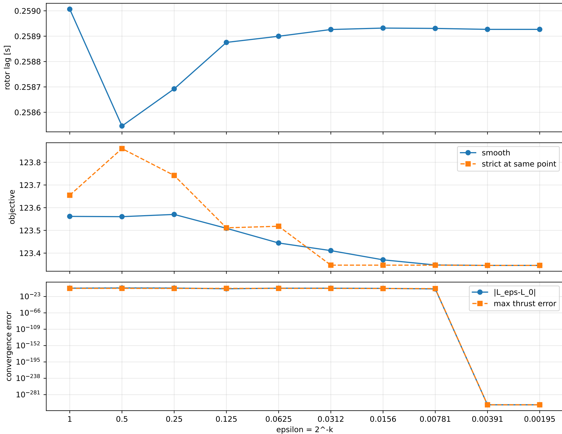
gimbal_command_replay: smooth-to-strict continuation
