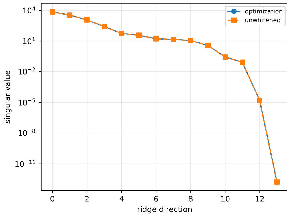
gimbal_command_replay: ridge spectrum (rank 13, nullity 1, ||v||=1.6e-13 )
