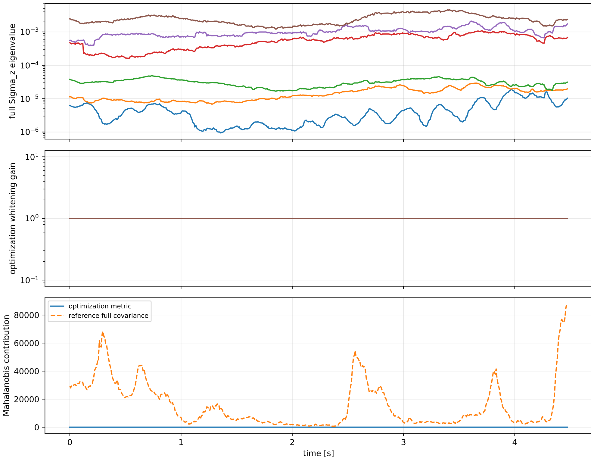
gimbal_measured_linear: optimization vs reference covariance
