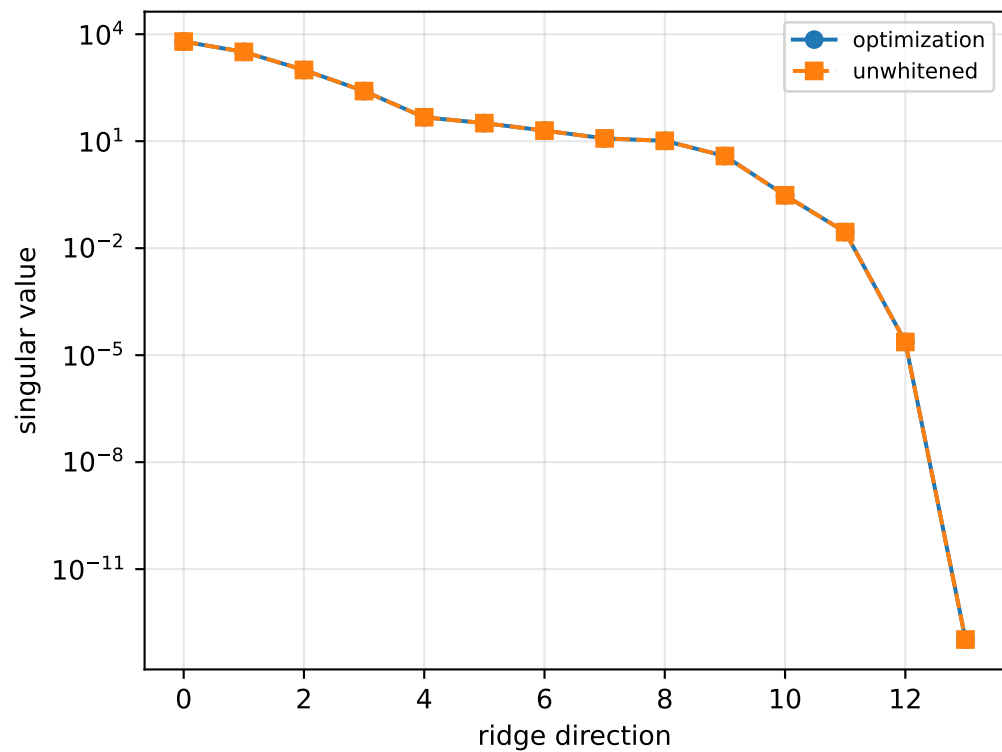
gimbal_measured_linear: ridge spectrum (rank 13, nullity 1, ||\mathbf{J}\mathbf{v}||=1.4\text{e-}13 )
