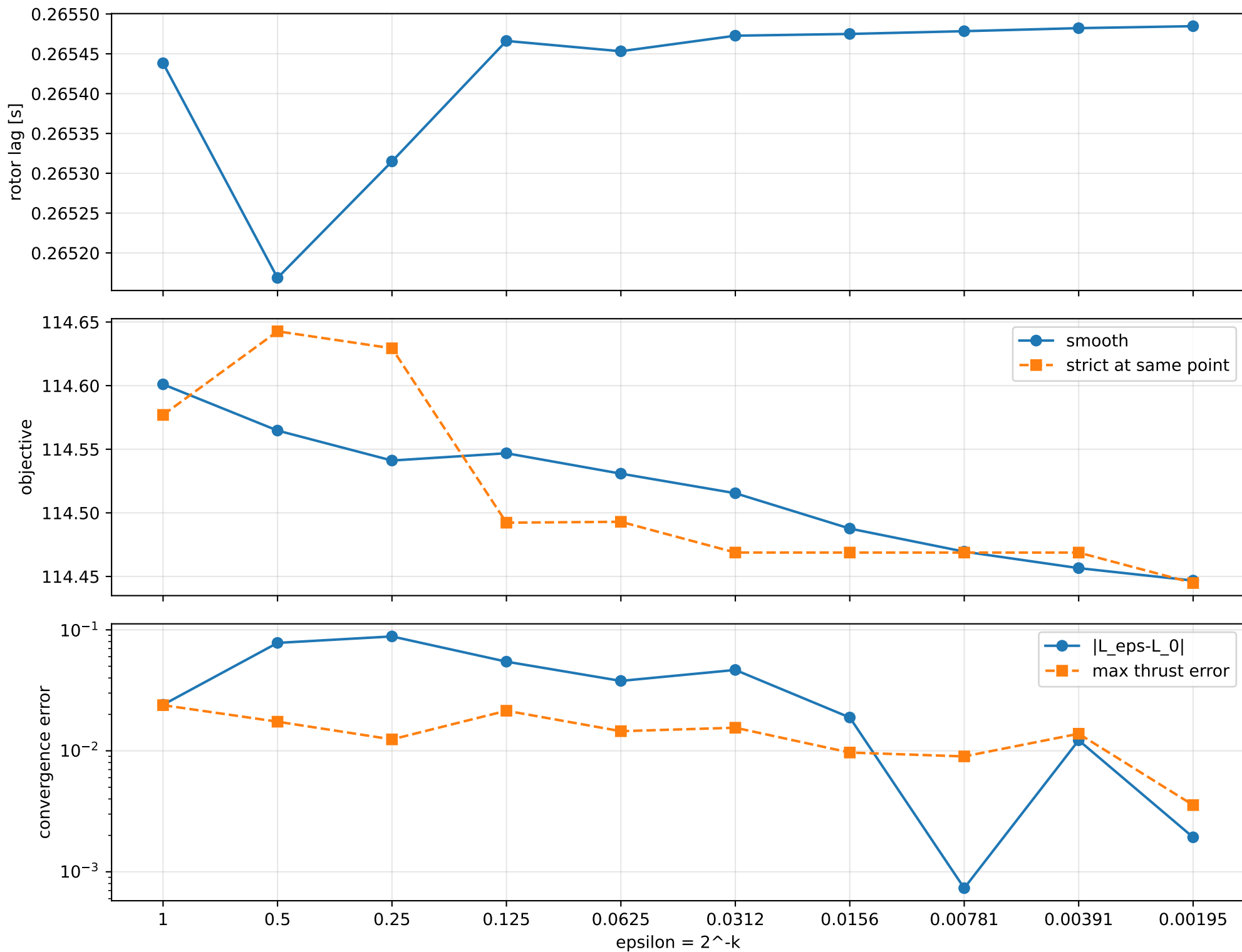
gimbal_measured_linear: smooth-to-strict continuation
