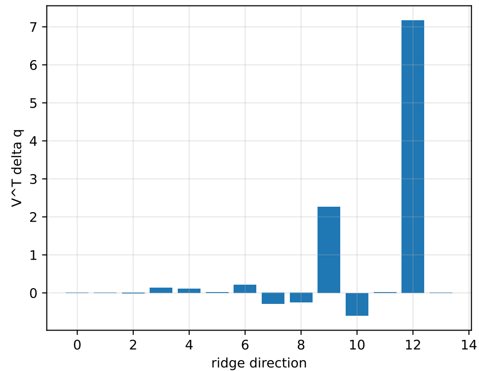
gimbal_measured_linear: ridge spectrum (rank 13, nullity 1, ||\mathbf{J}\mathbf{v}||=1.4\text{e-}13 )
