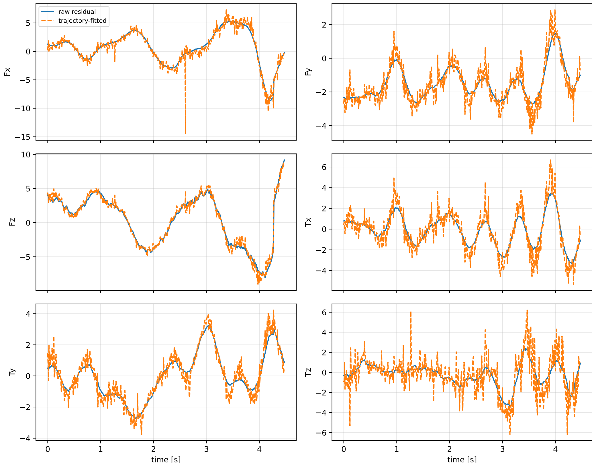
lag_fixed_one_period: wrench / closure (force max 3.29\text{e-}14 , torque max 2.66\text{e-}15 )
