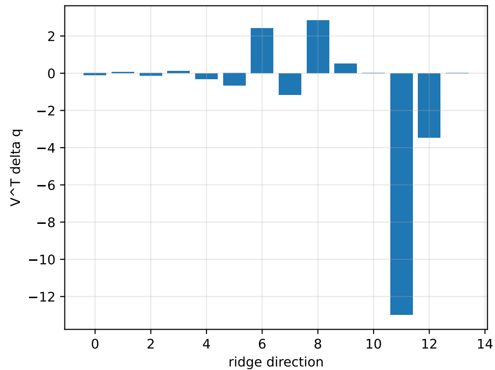
lag_fixed_one_period: ridge spectrum (rank 13, nullity 1, ||\mathbf{J}\mathbf{v}||=6.02\text{e-}14 )
