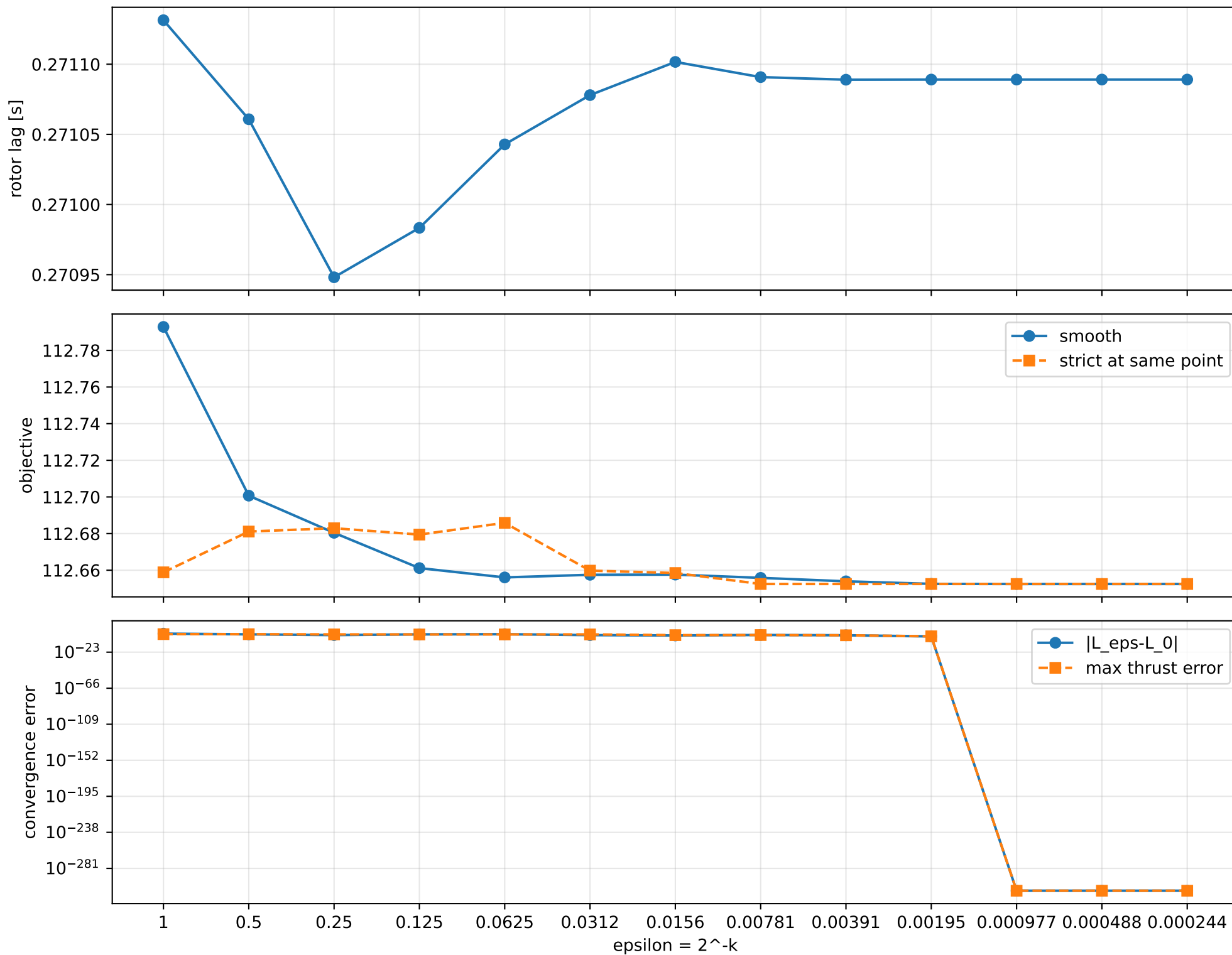
lag_pow2_depth_12: smooth-to-strict continuation
