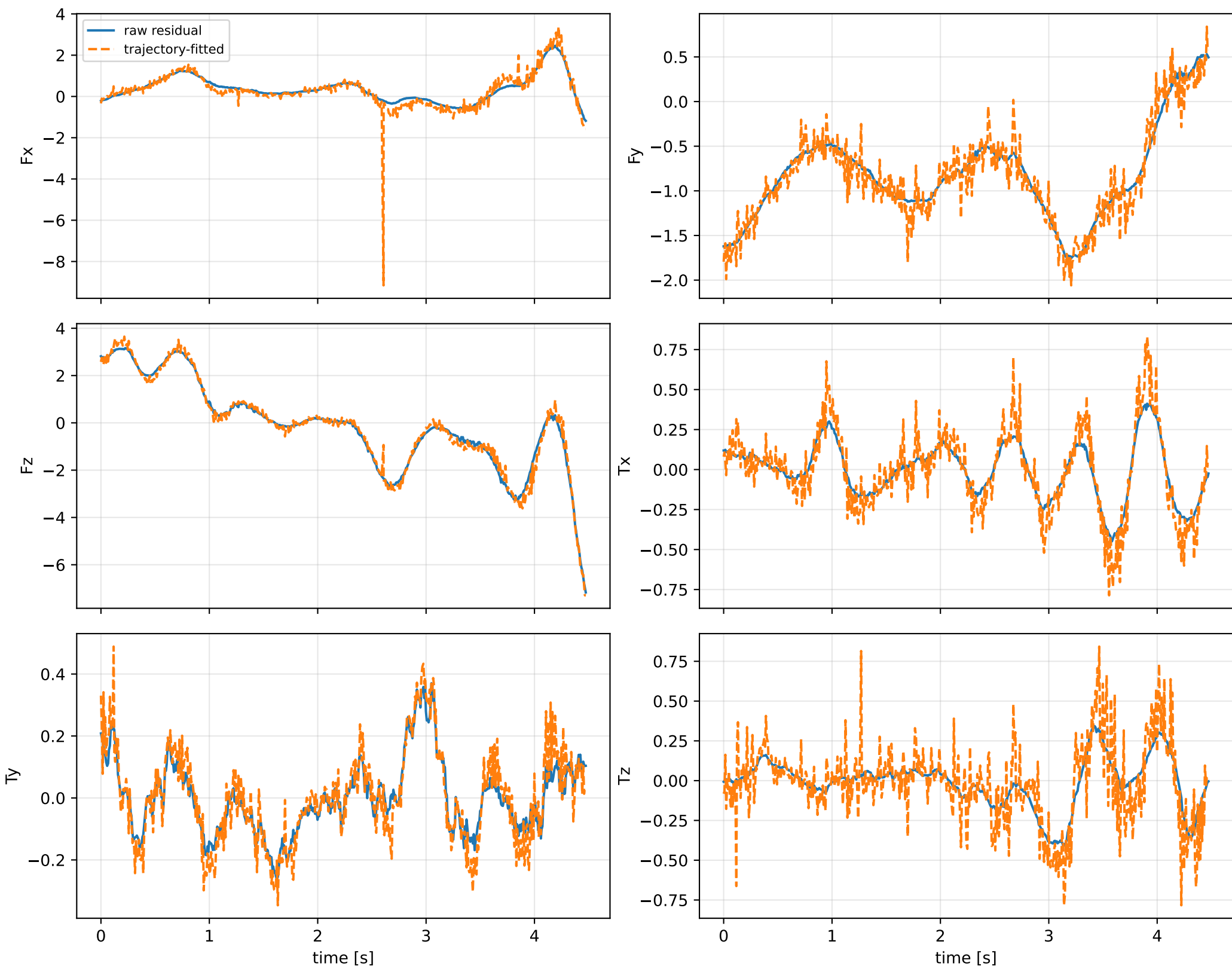
lag_pow2_depth_12: wrench / closure (force max 2.3\text{e-}14 , torque max 5.41\text{e-}16 )
