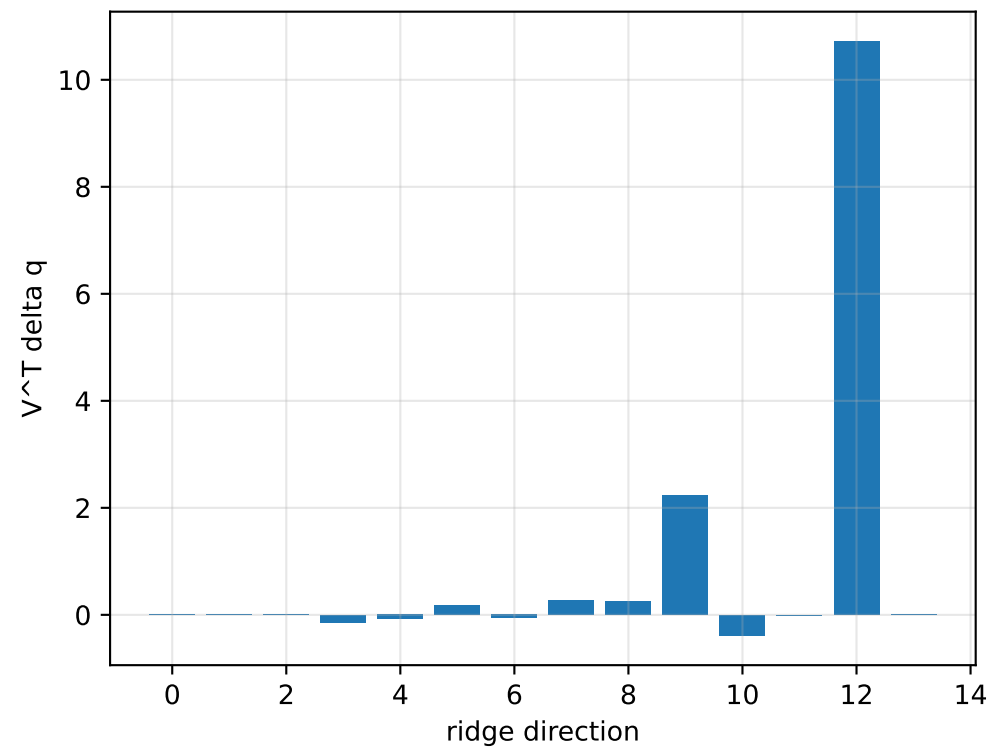
lag_pow2_depth_12: ridge spectrum (rank 13, nullity 1, ||\mathbf{J}\mathbf{v}||=1.56\text{e-}13 )
