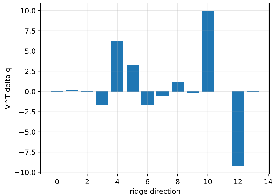
cov_full_no_R_uncertainty_in_s: ridge spectrum (rank 13, nullity 1, ||jv||=4.36e-10)
