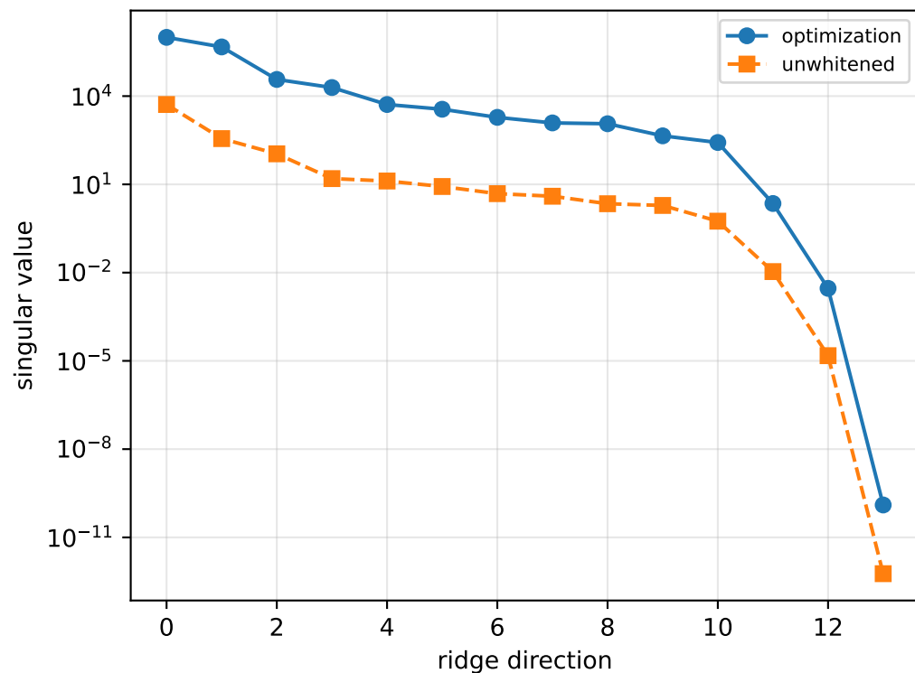
cov_full_no_R_uncertainty_in_s: ridge spectrum (rank 13, nullity 1, ||jv||=4.36e-10)
