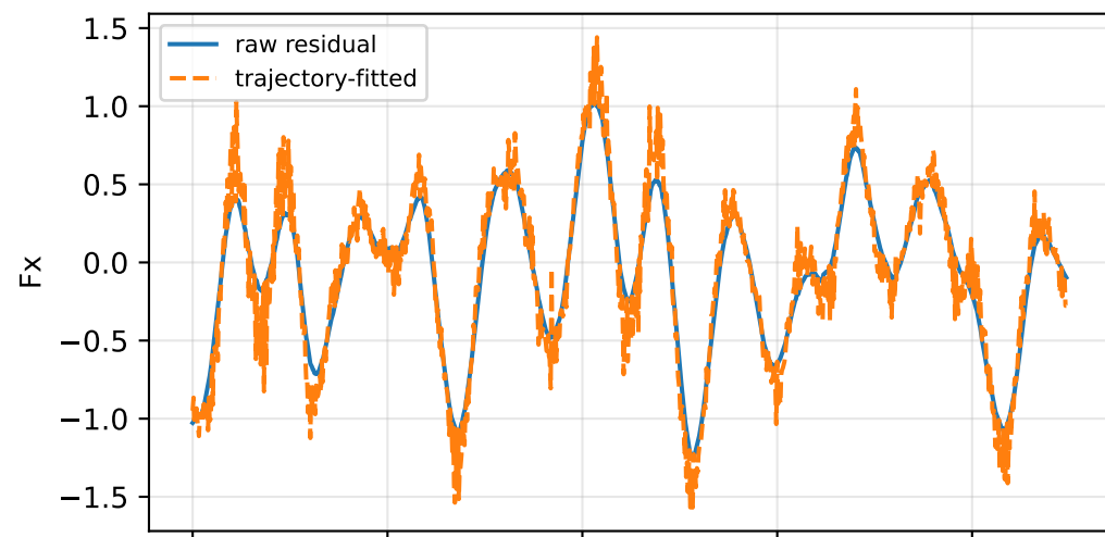
cov_full_no_R_uncertainty_in_s: wrench / closure (force max 3.66\text{e-}15 , torque max 6.39\text{e-}14 )
