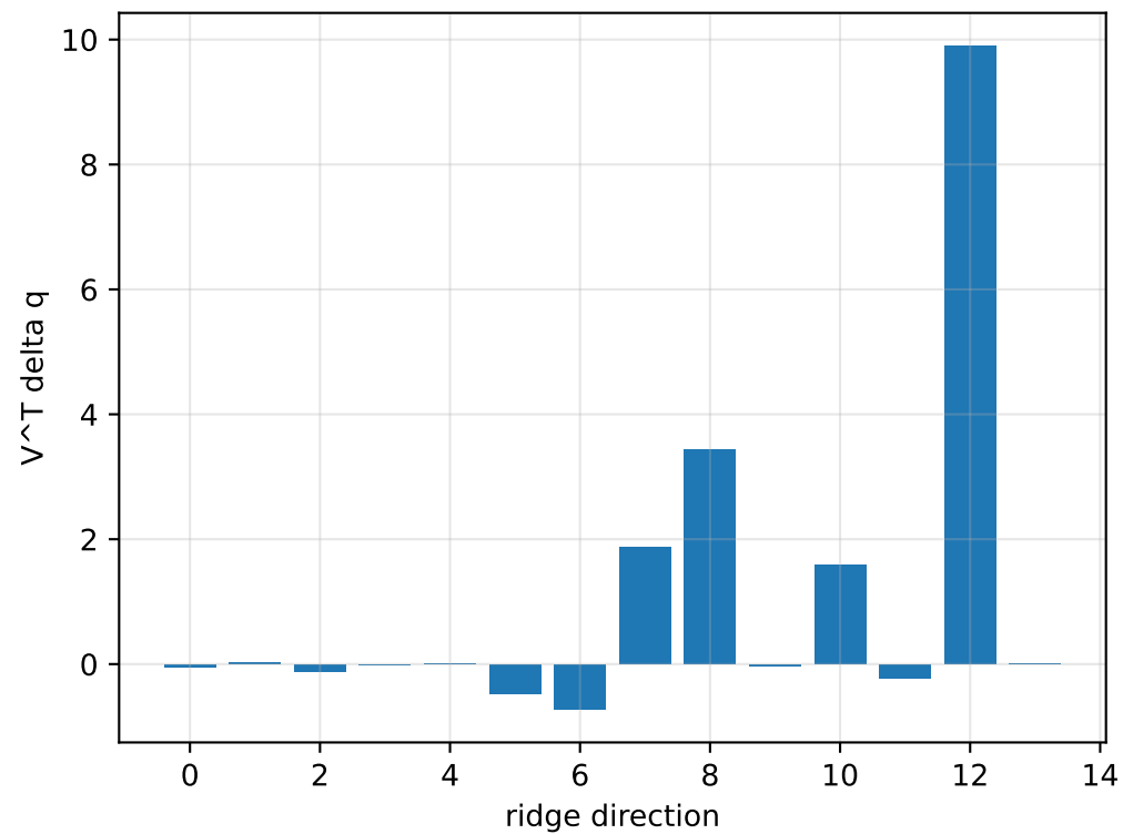
cov_full_no_position_rotation_cross: ridge spectrum (rank 13, nullity 1, ||jv||=5.67e-11)
