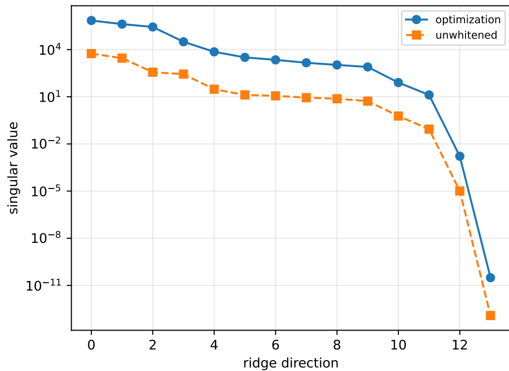
cov_full_no_position_rotation_cross: ridge spectrum (rank 13, nullity 1, ||jv||=5.67e-11)
