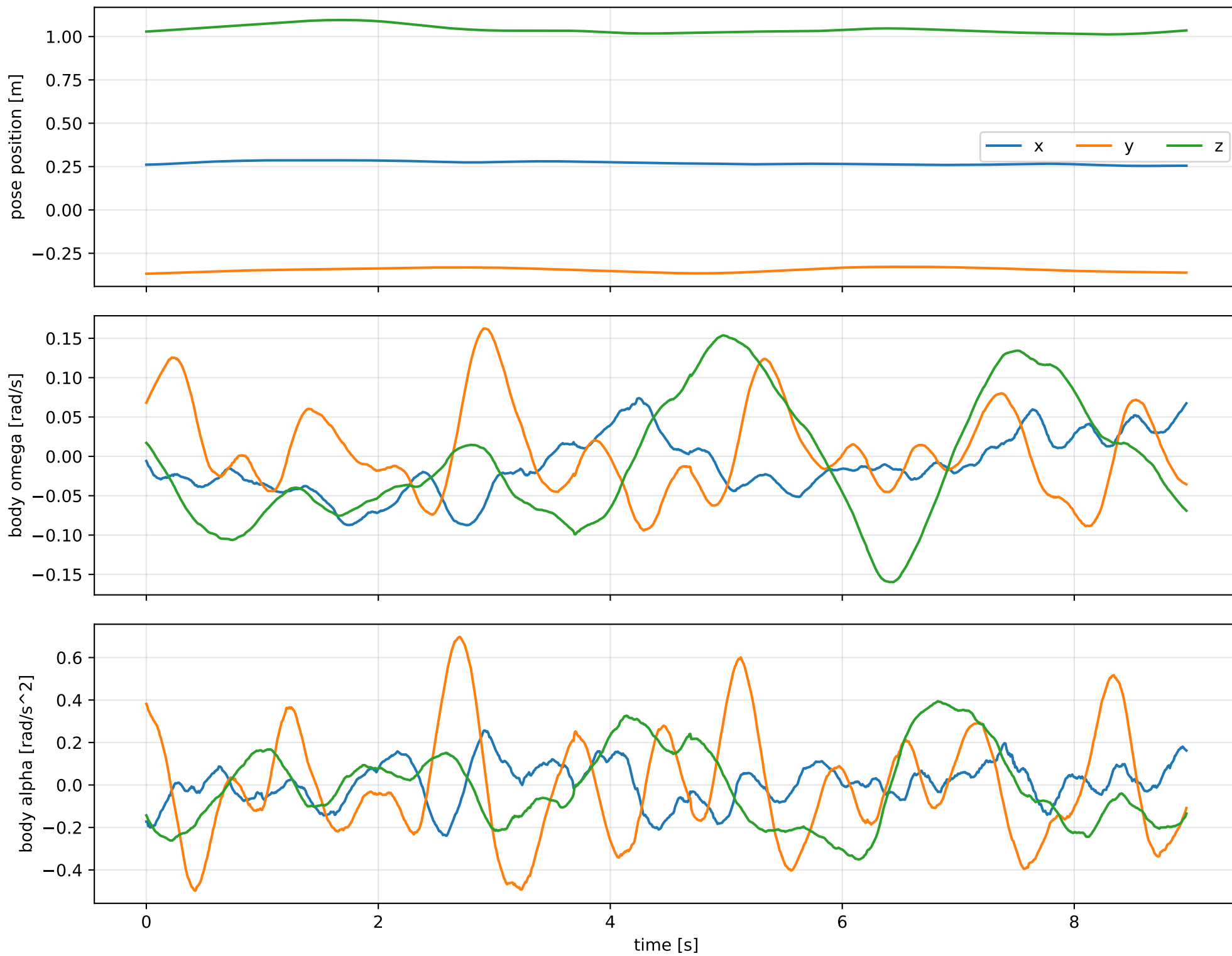
cov_global_full: SG trajectory and derived motion
