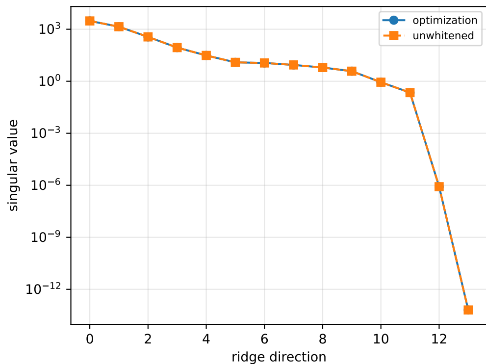
gimbal_command_replay: ridge spectrum (rank 13, nullity 1, ||\mathbf{J}\mathbf{v}||=7.68\text{e-}14 )
