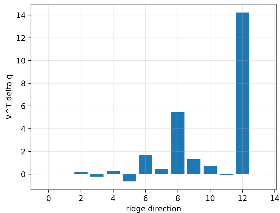
kkt_scale_negative: ridge spectrum (rank 13, nullity 1, ||jv||=8.35e-14 )
