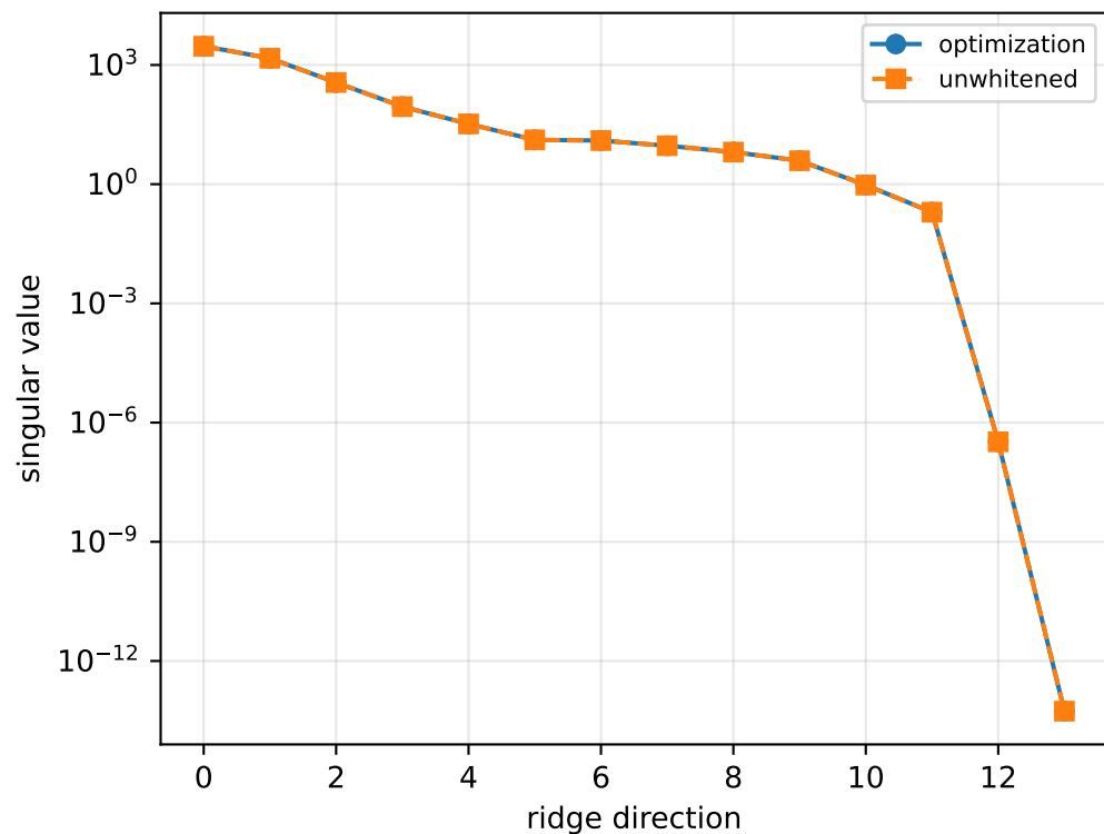
kkt_scale_positive: ridge spectrum (rank 13, nullity 1, ||\mathbf{J}\mathbf{v}||=7.97\text{e-}14 )
