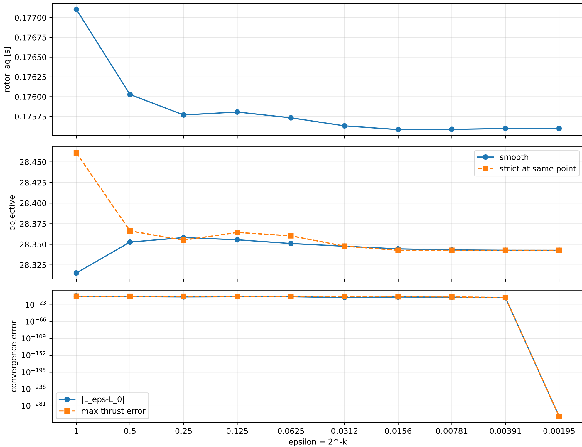
kkt_scale_positive: smooth-to-strict continuation
