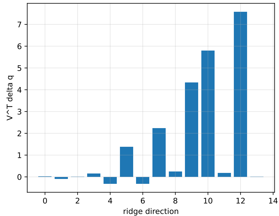
lag_fixed_one_period: ridge spectrum (rank 13, nullity 1, ||Jv||=5.63e-14)
