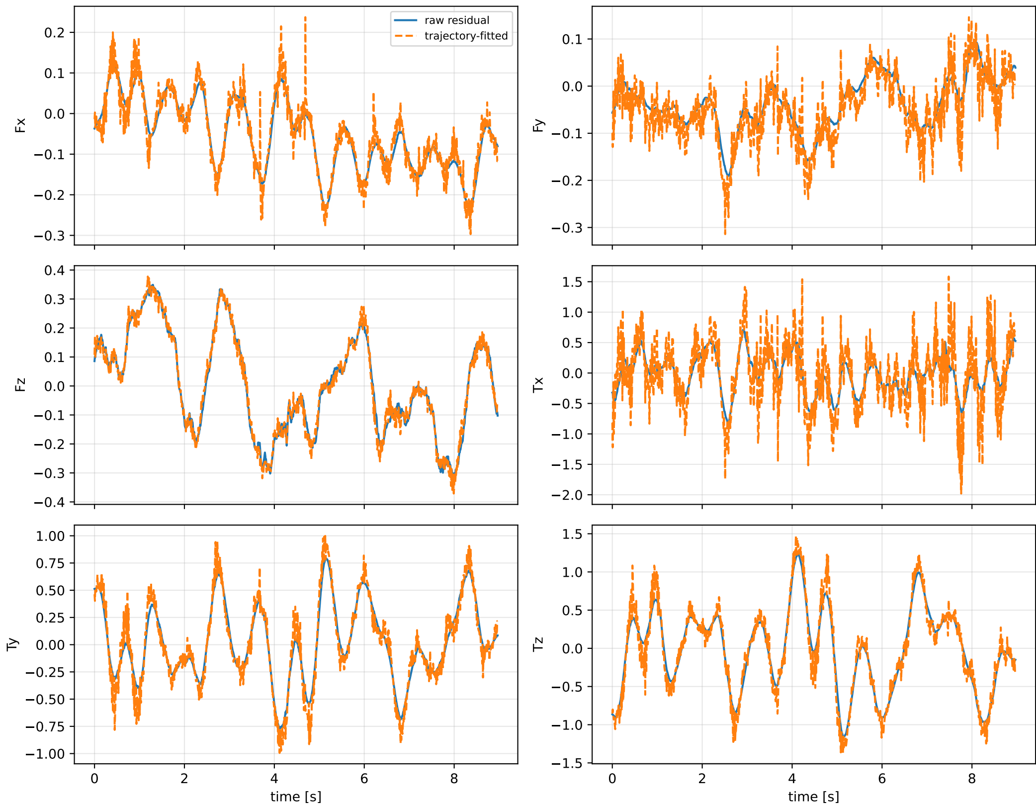
lag_fixed_one_period: wrench / closure (force max 5.5\text{e-}15 , torque max 3.33\text{e-}16 )
