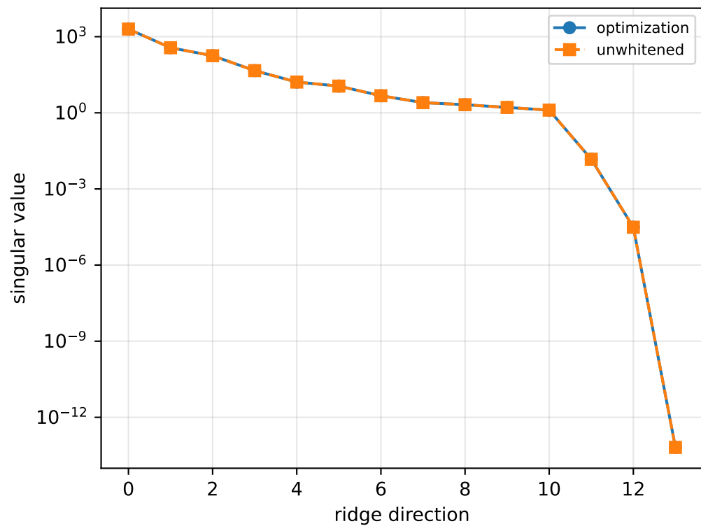
lag_fixed_one_period: ridge spectrum (rank 13, nullity 1, ||Jv||=5.63e-14)
