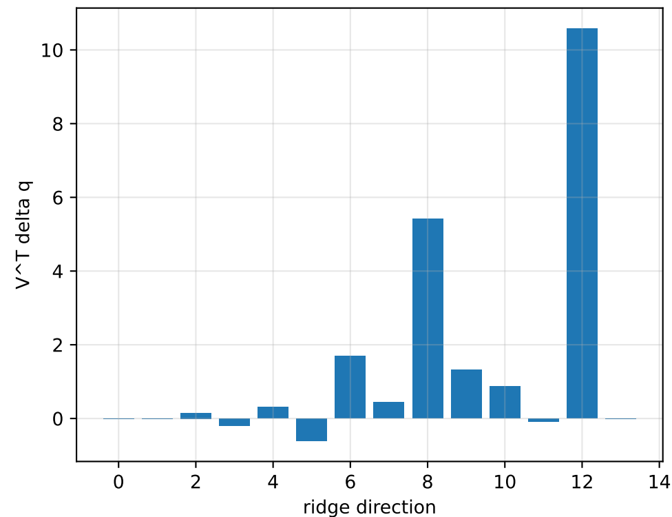
lag_legacy_smooth_schedule: ridge spectrum (rank 13, nullity 1, ||Jv||=7.95e-14)
