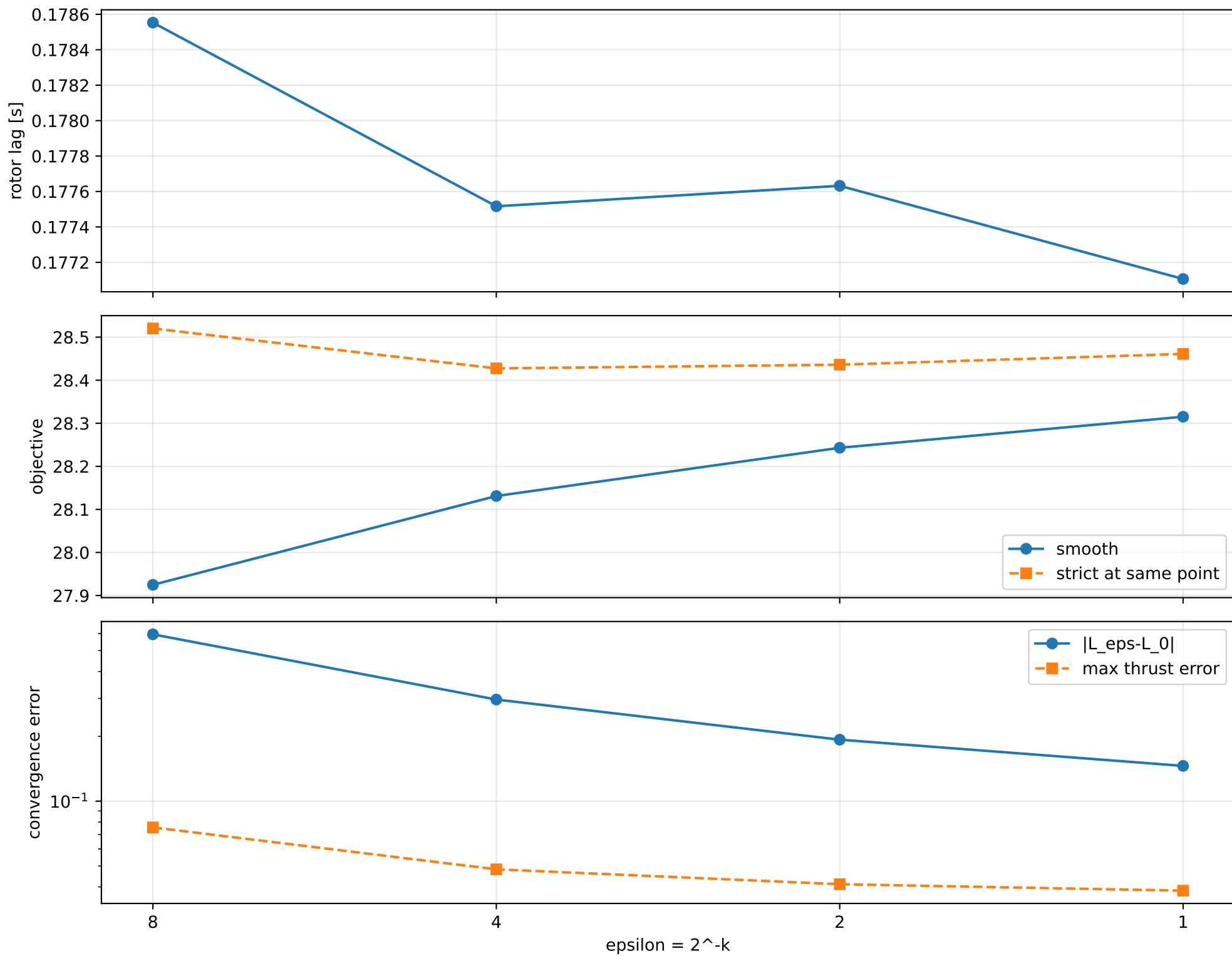
lag_legacy_smooth_schedule: smooth-to-strict continuation
