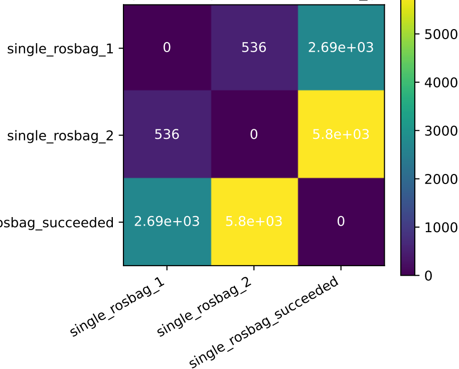
pairwise quotient distance d_{ij}
