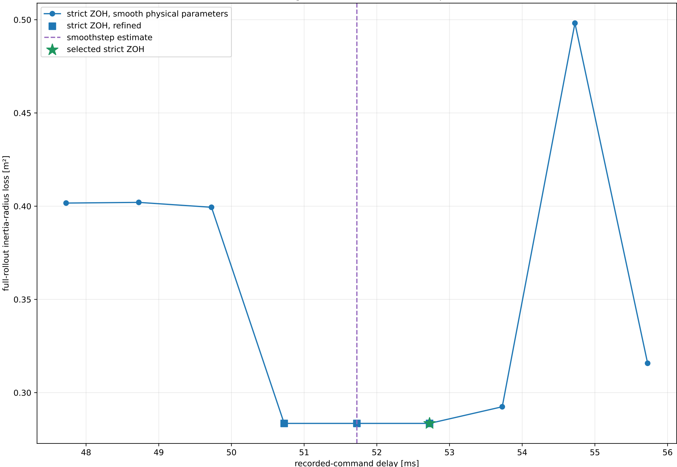
Smooth lag search and strict-ZOH local polish
