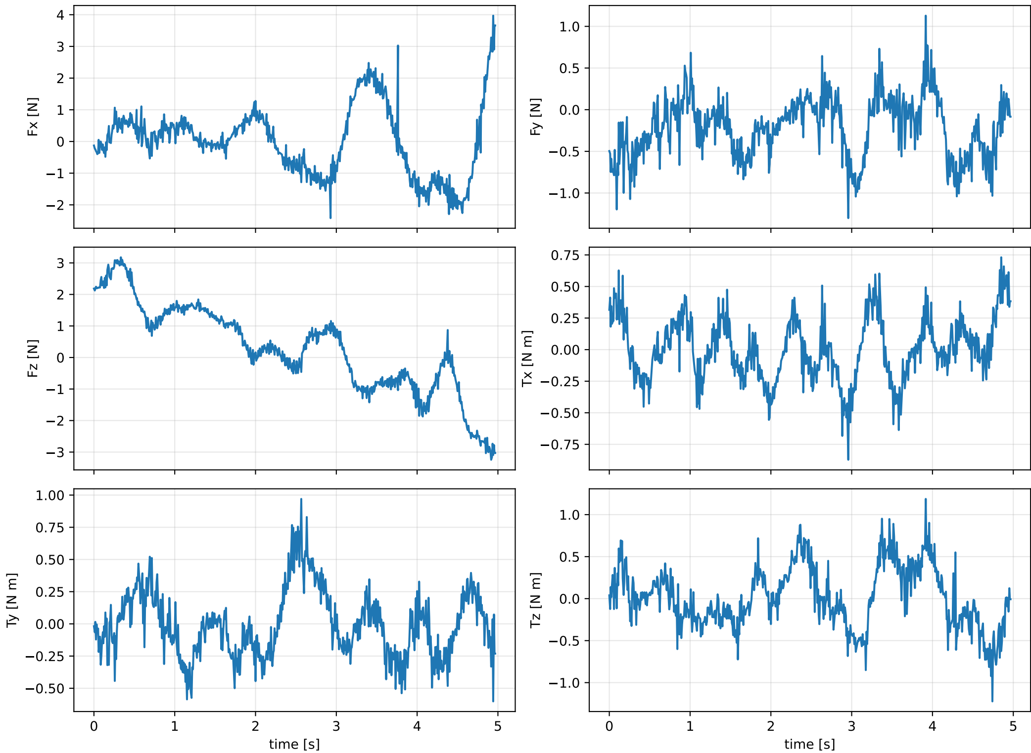
failure1: trajectory-fitted external wrench used by replay
