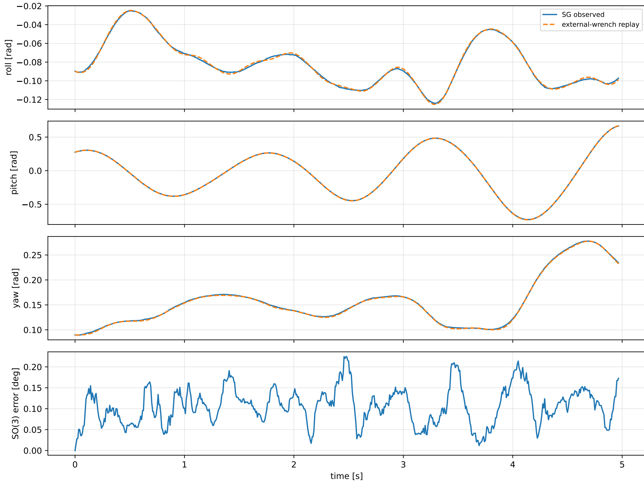
failure1: body-orientation replay; geodesic RMS 0.1153 deg
