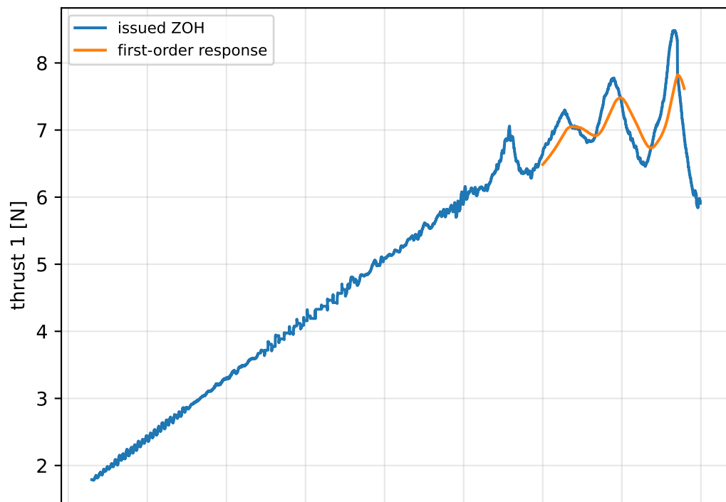
failure2: command and fitted first-order thrust, tau=0.398608 s
