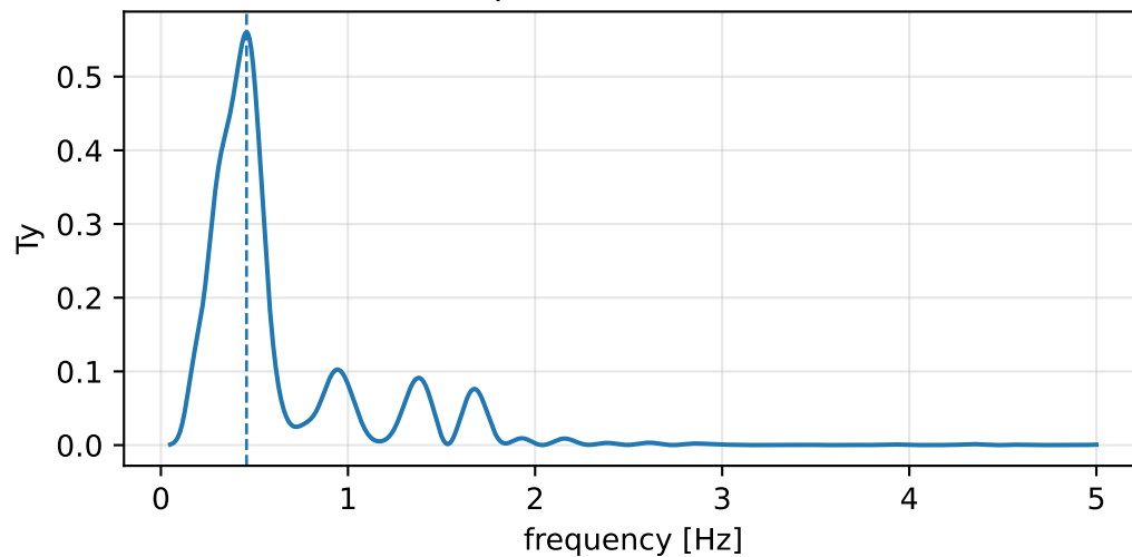
peak 0.4577 Hz
