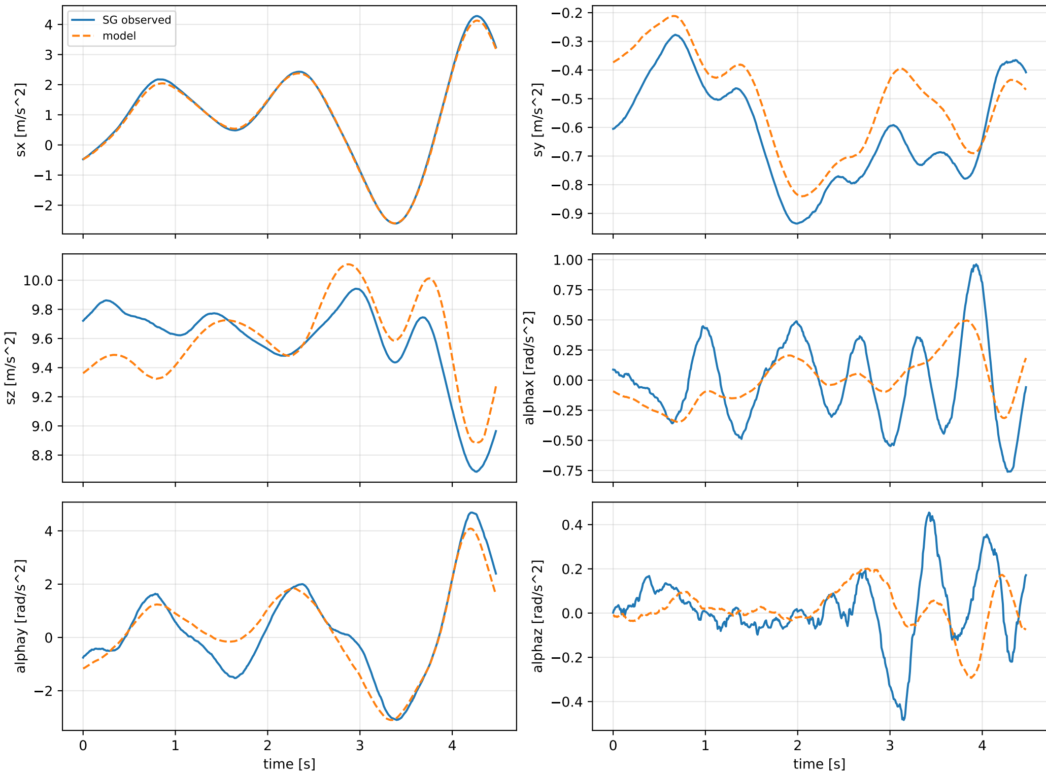
failure2: acceleration objective
