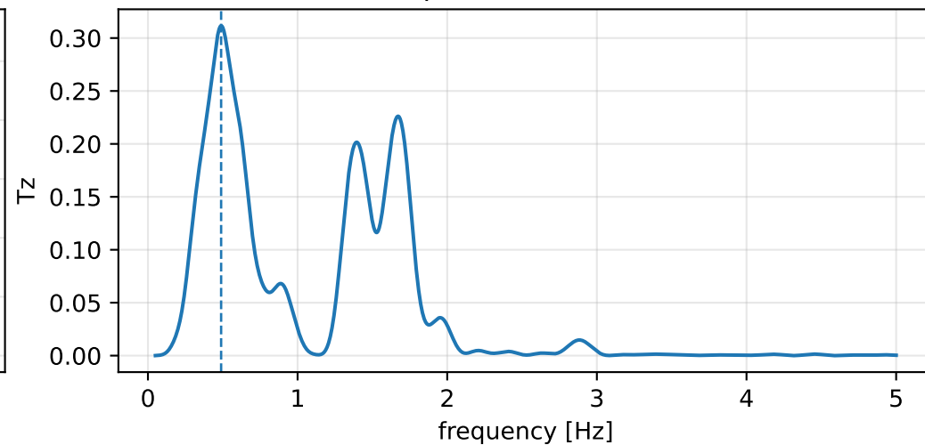
peak 0.489 Hz
