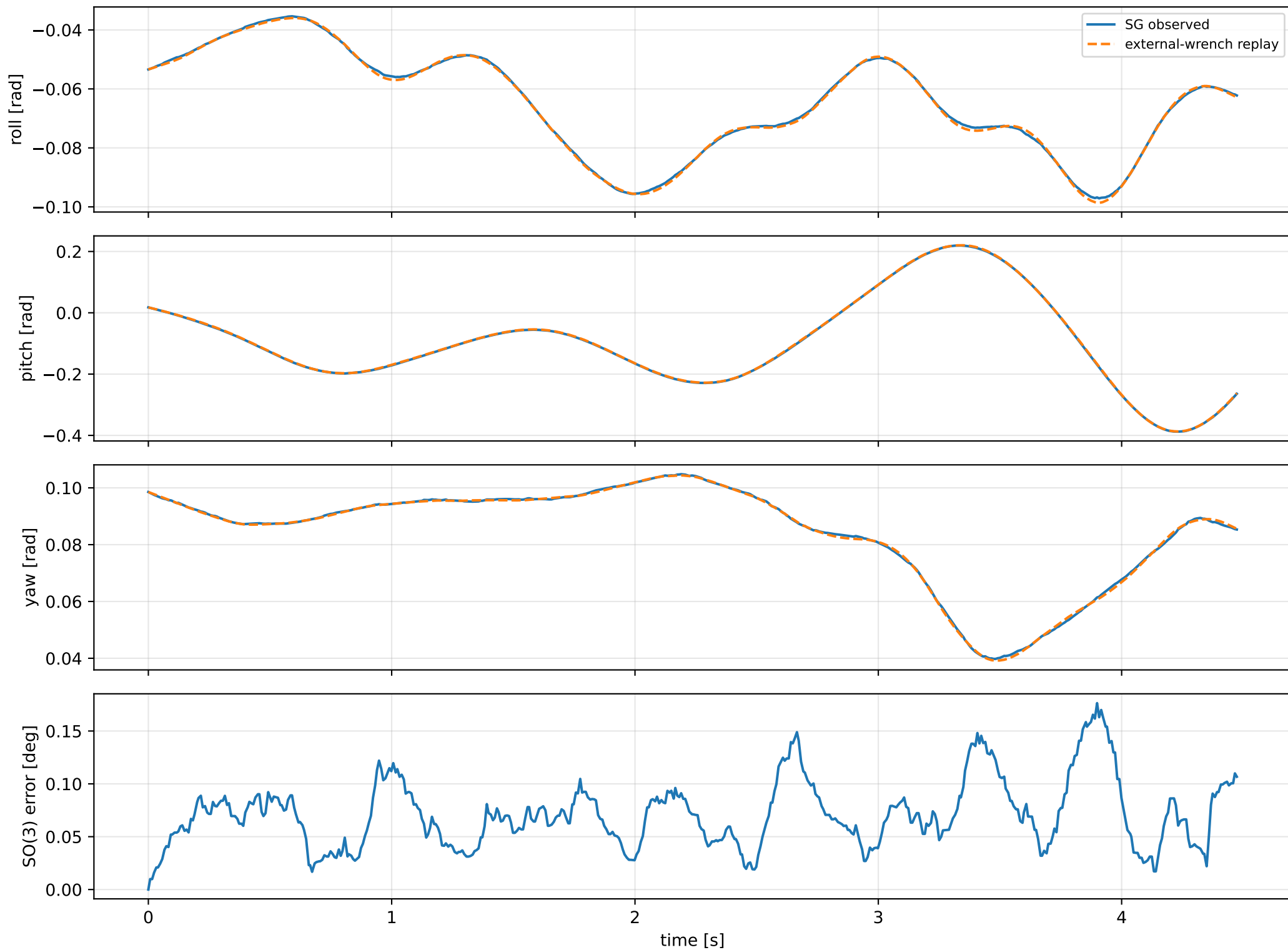
failure2: body-orientation replay; geodesic RMS 0.07771 deg
