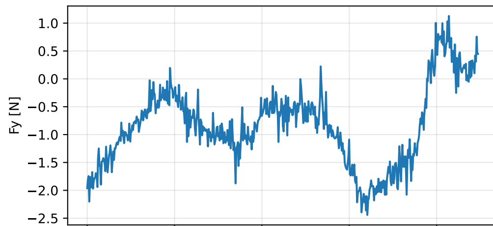
failure2: trajectory-fitted external wrench used by replay
