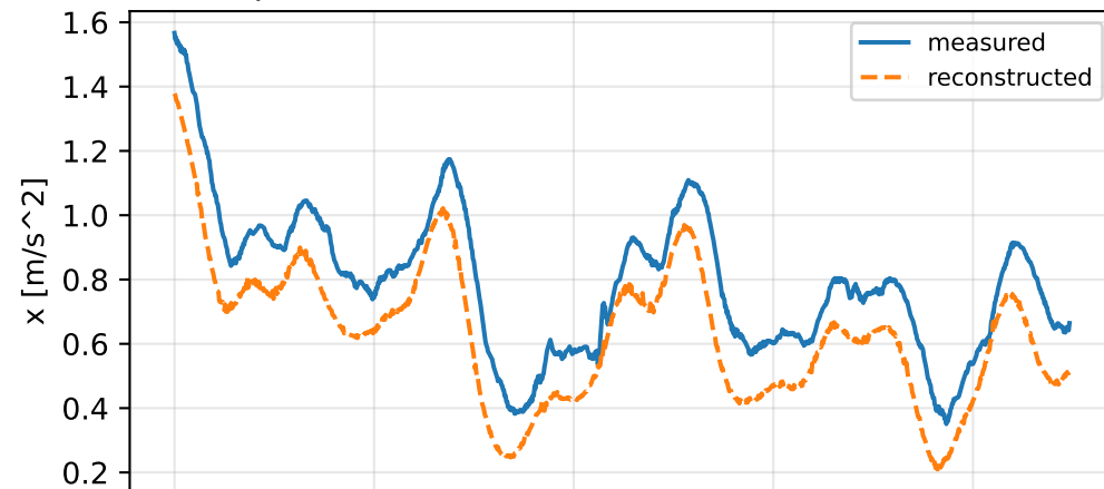
specific-force RMSE [0.168 0.0507 0.0323]
