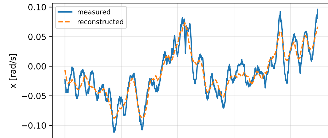
gyro RMSE [0.0142 0.0128 0.0059]
