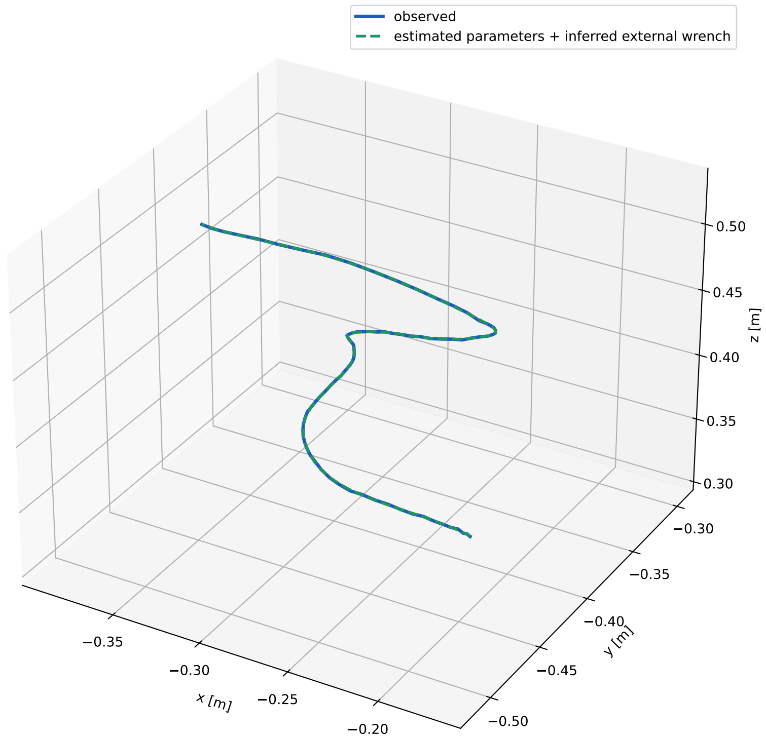
Observed and reconstructed 3D trajectory
