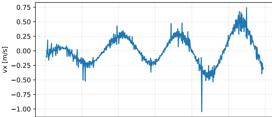
Translational derivatives at raw centered evaluation times
