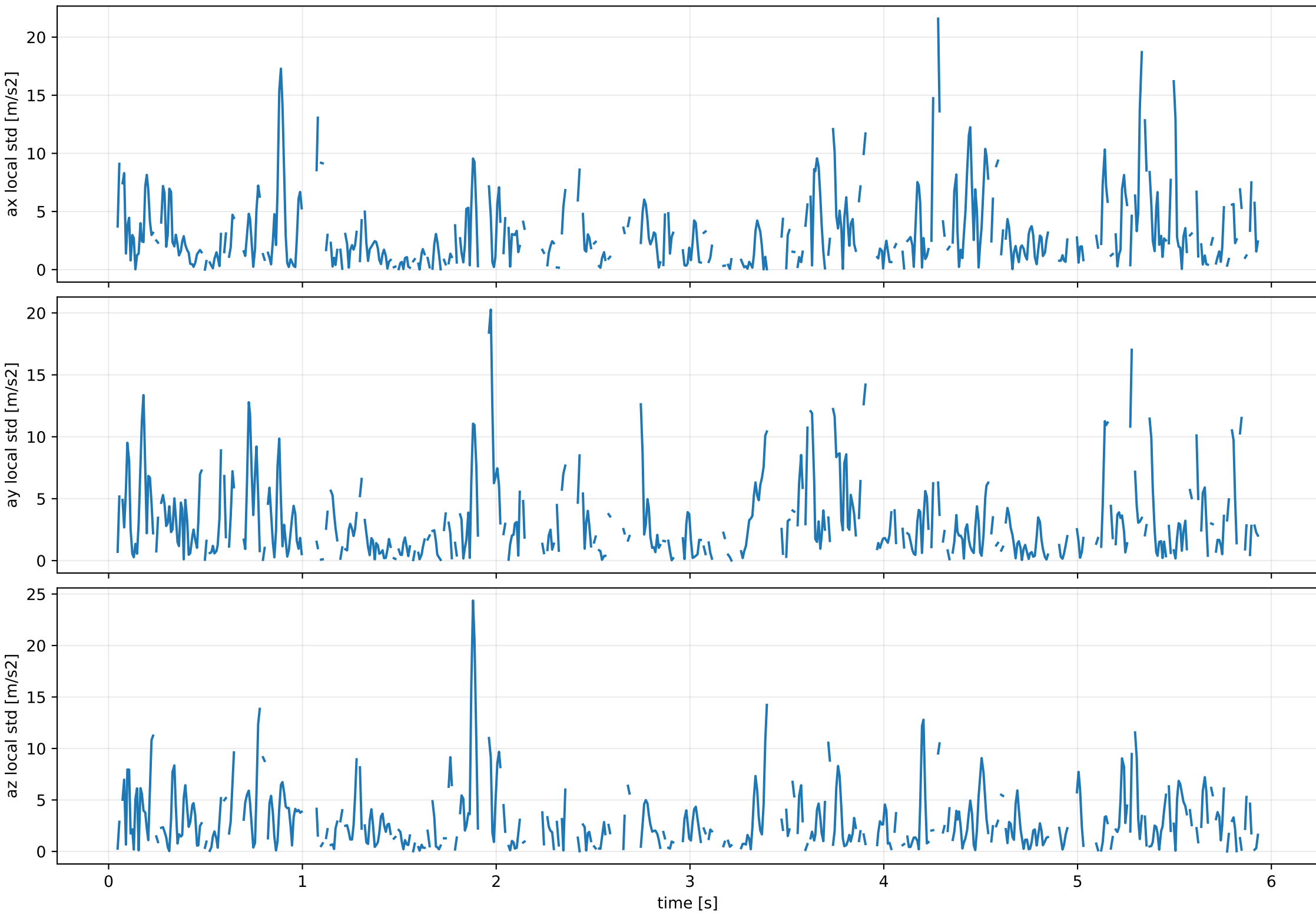
Translation second-derivative covariance from local LS residuals
