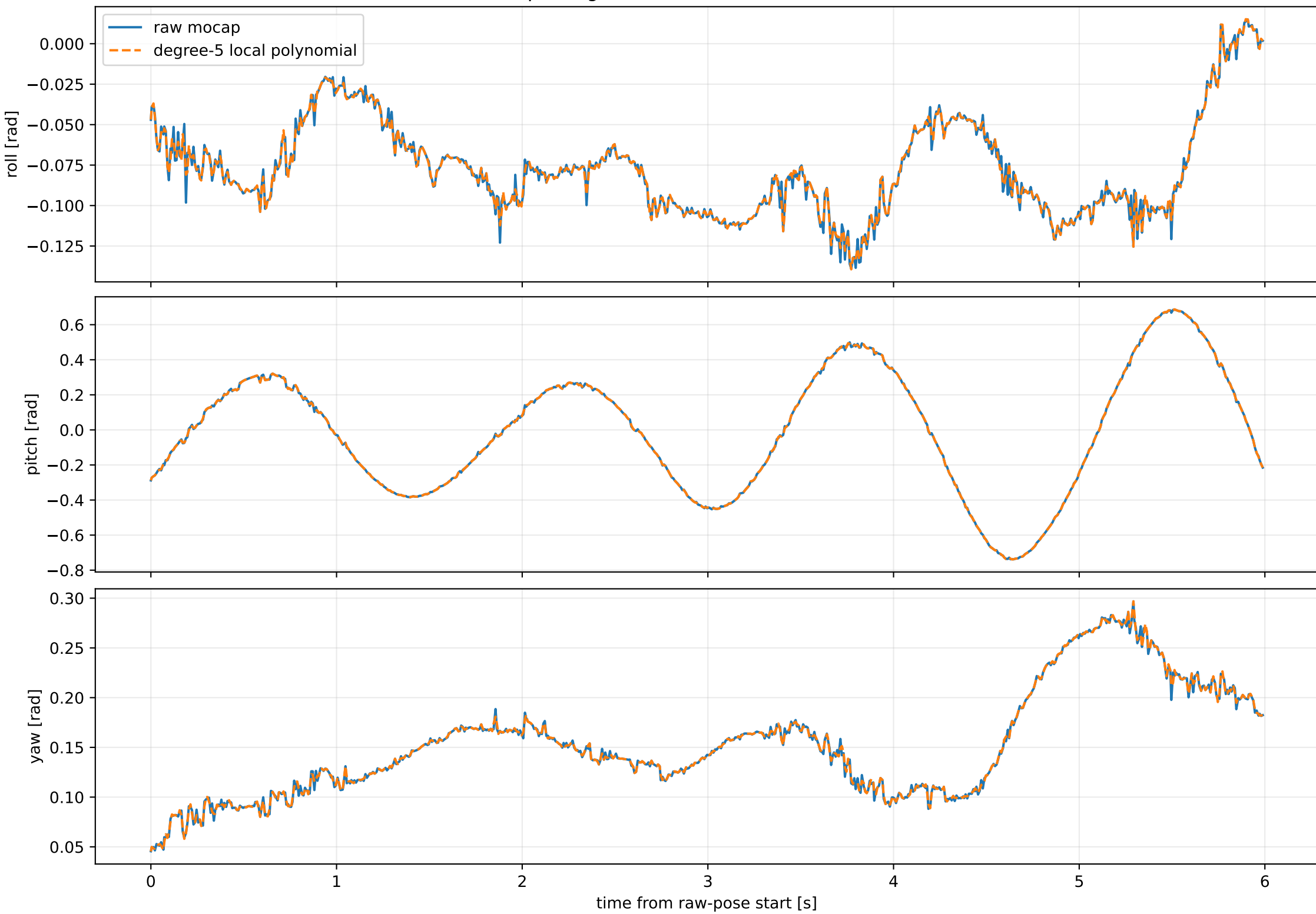
Raw mocap and geometric-SG orientation; W=0.0528808s
