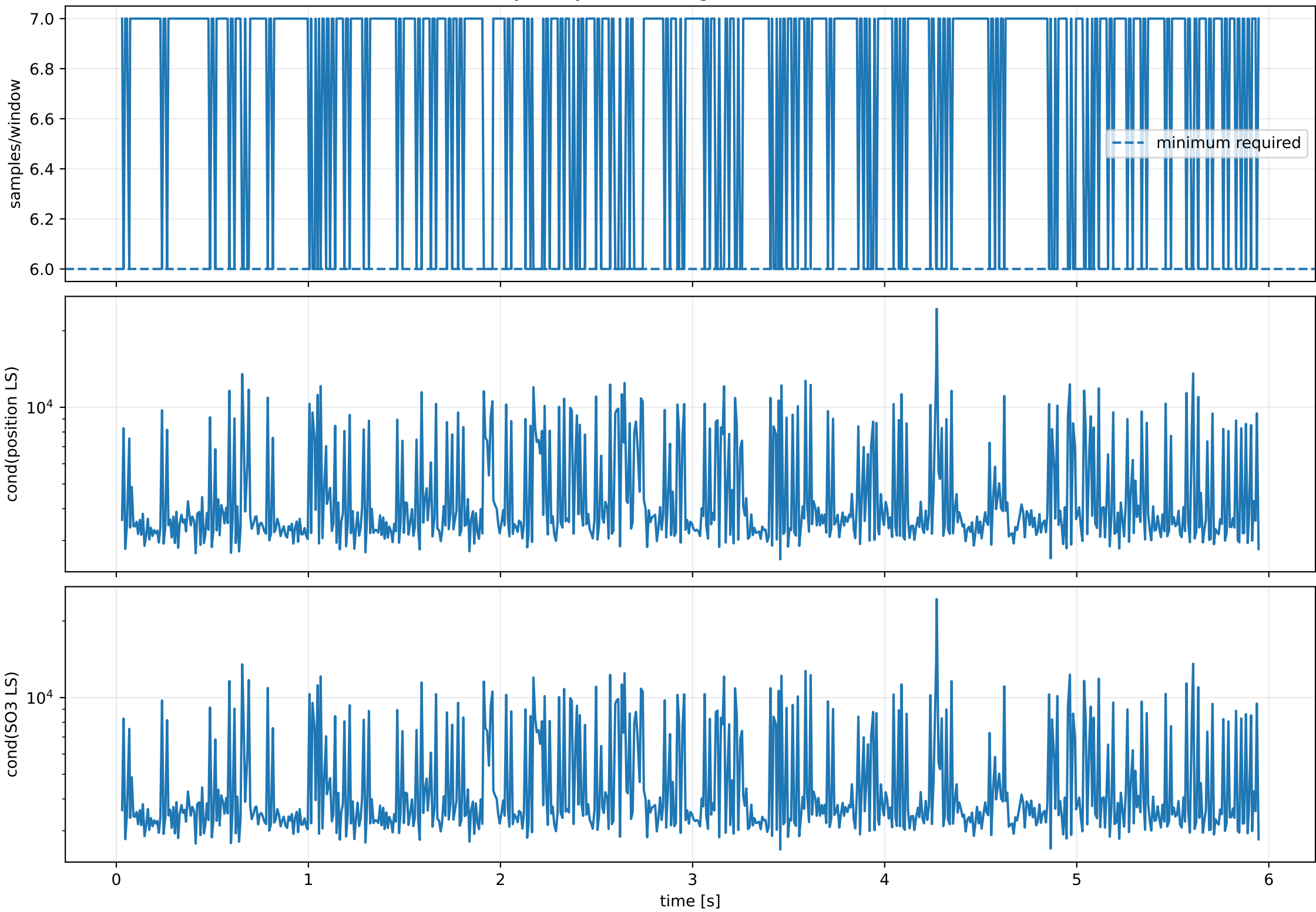
Savitzky-Golay window diagnostics; W=0.0528808s
