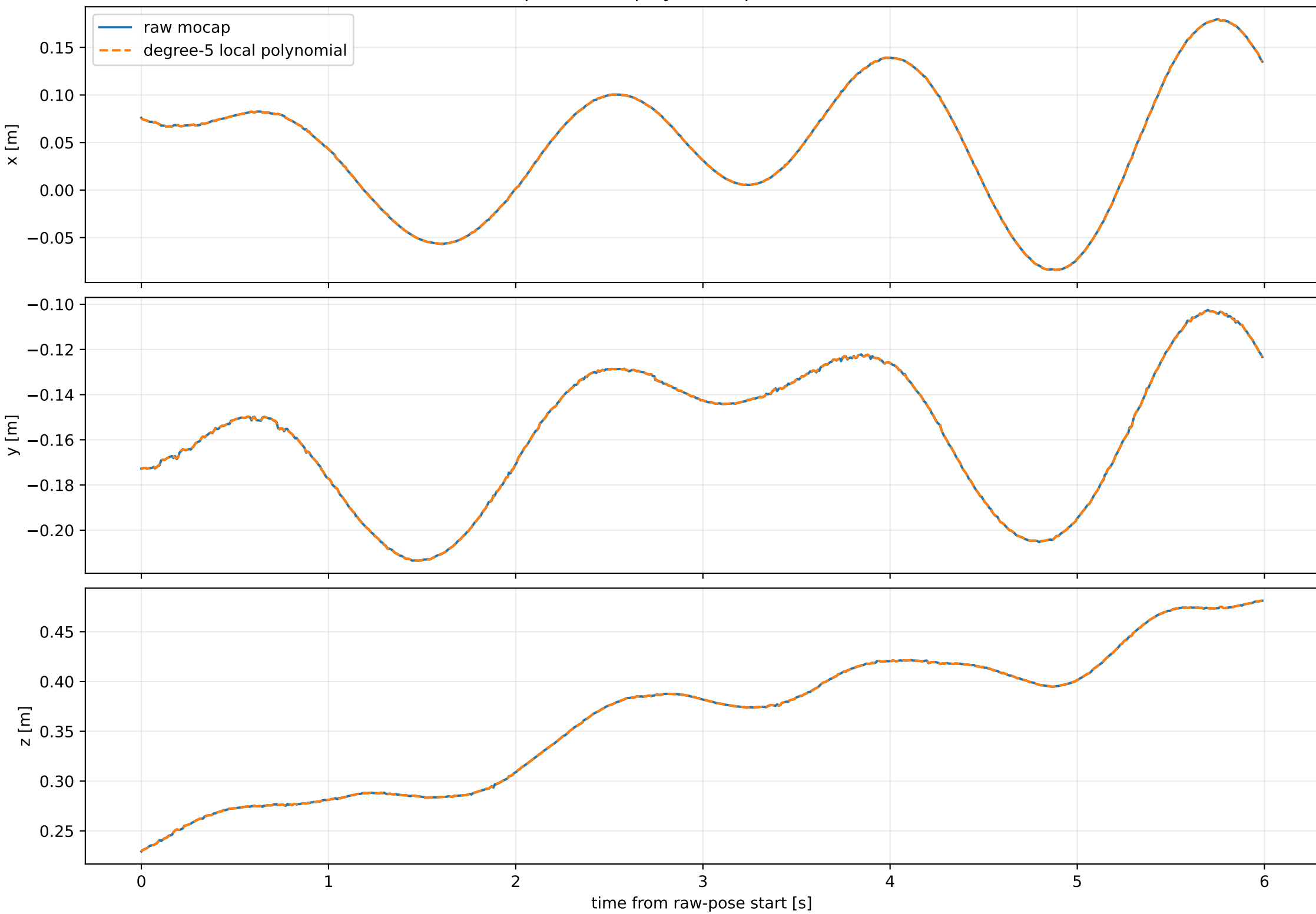
Raw mocap and local-polynomial position; W=0.0528808s
