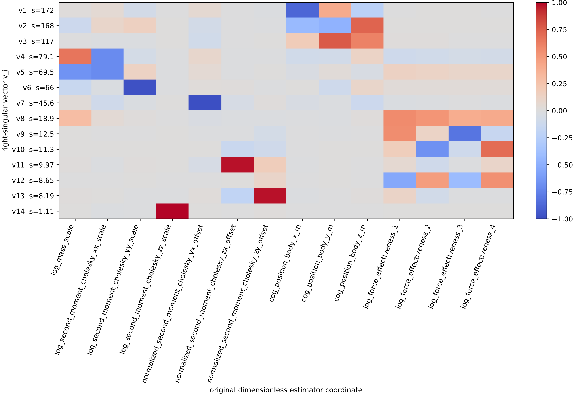
Signed right-singular vectors V^T A complete row may flip sign; relative signs inside the row matter
