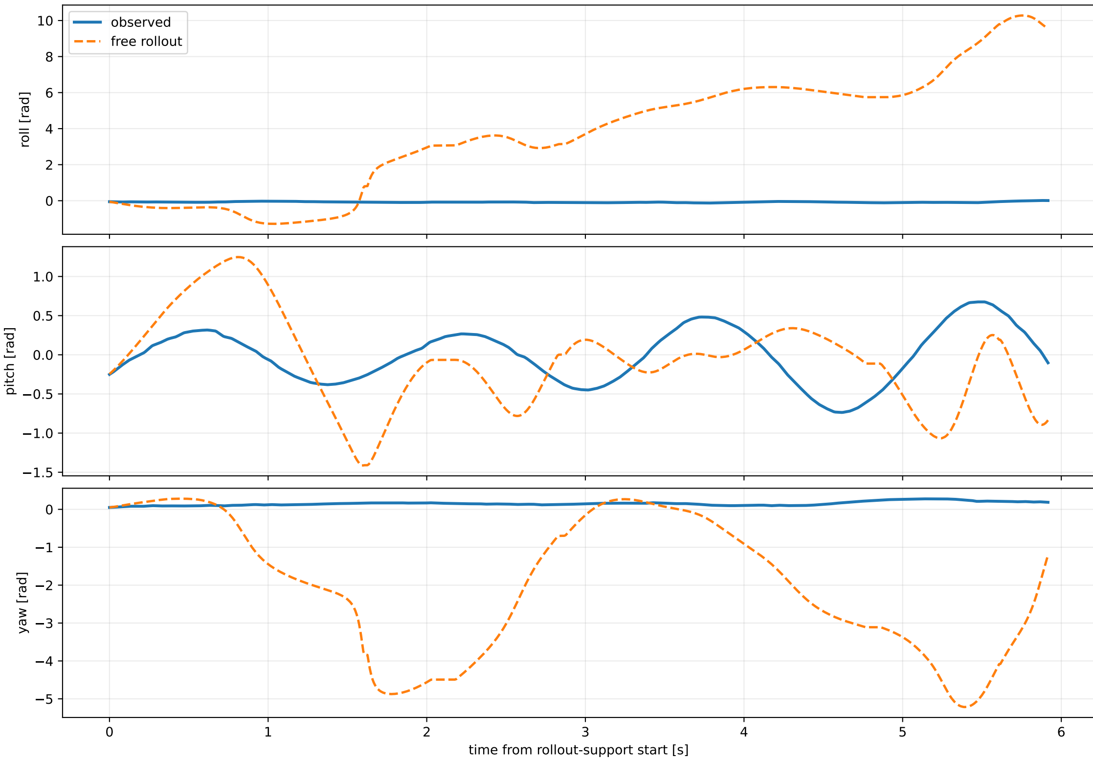
Observed and free-rollout sensor orientation
