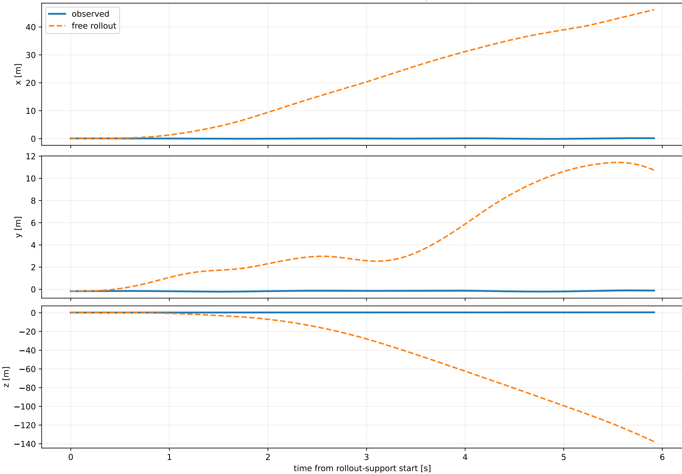
Observed and free-rollout sensor position
