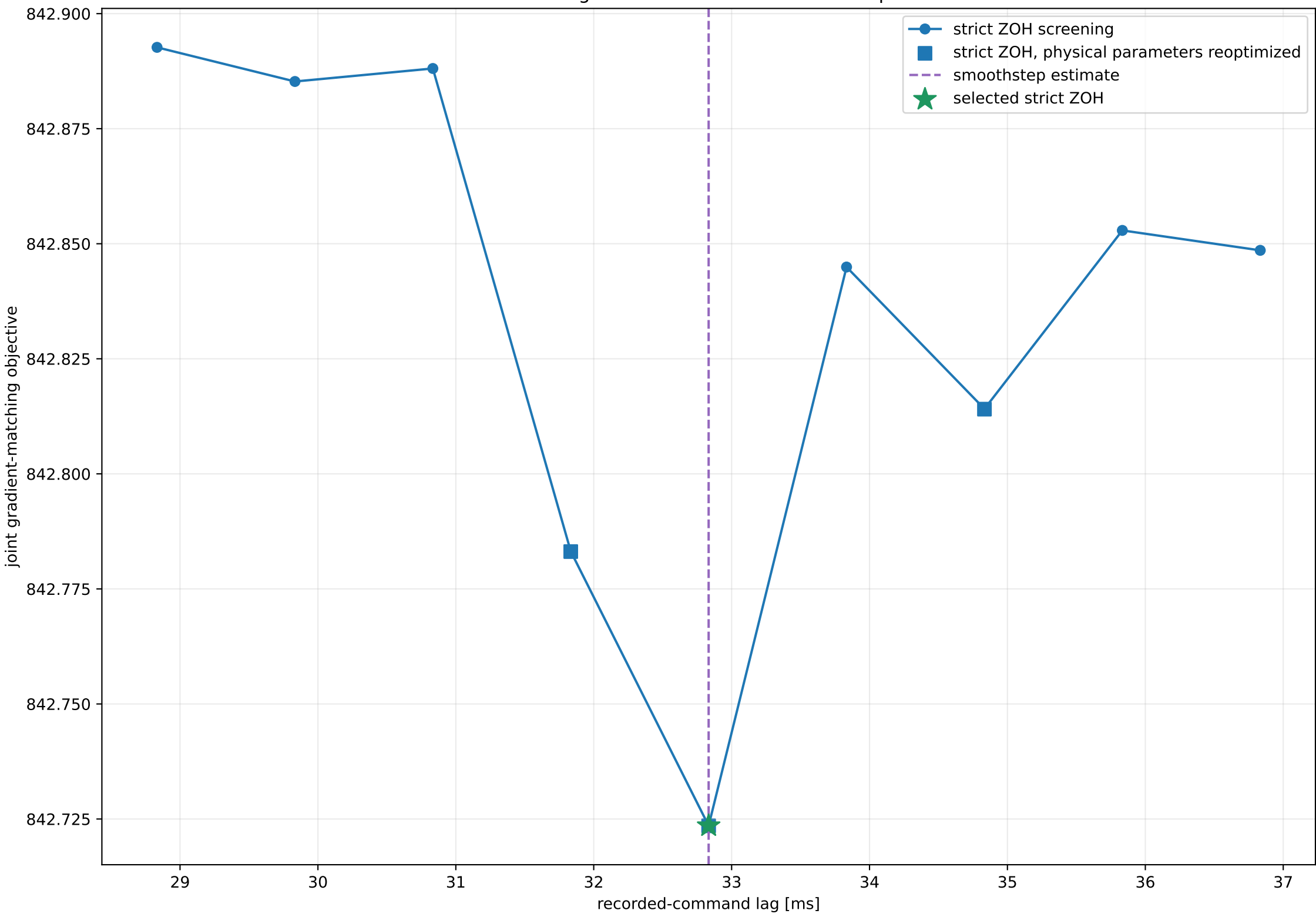
Smooth lag estimate and strict-ZOH local polish
