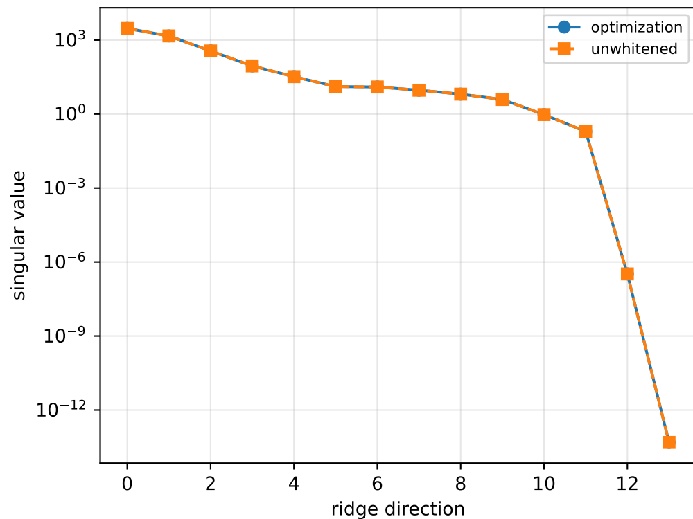
default: ridge spectrum (rank 13, nullity 1, ||\mathbf{J}\mathbf{v}||=7.94\text{e-}14 )
