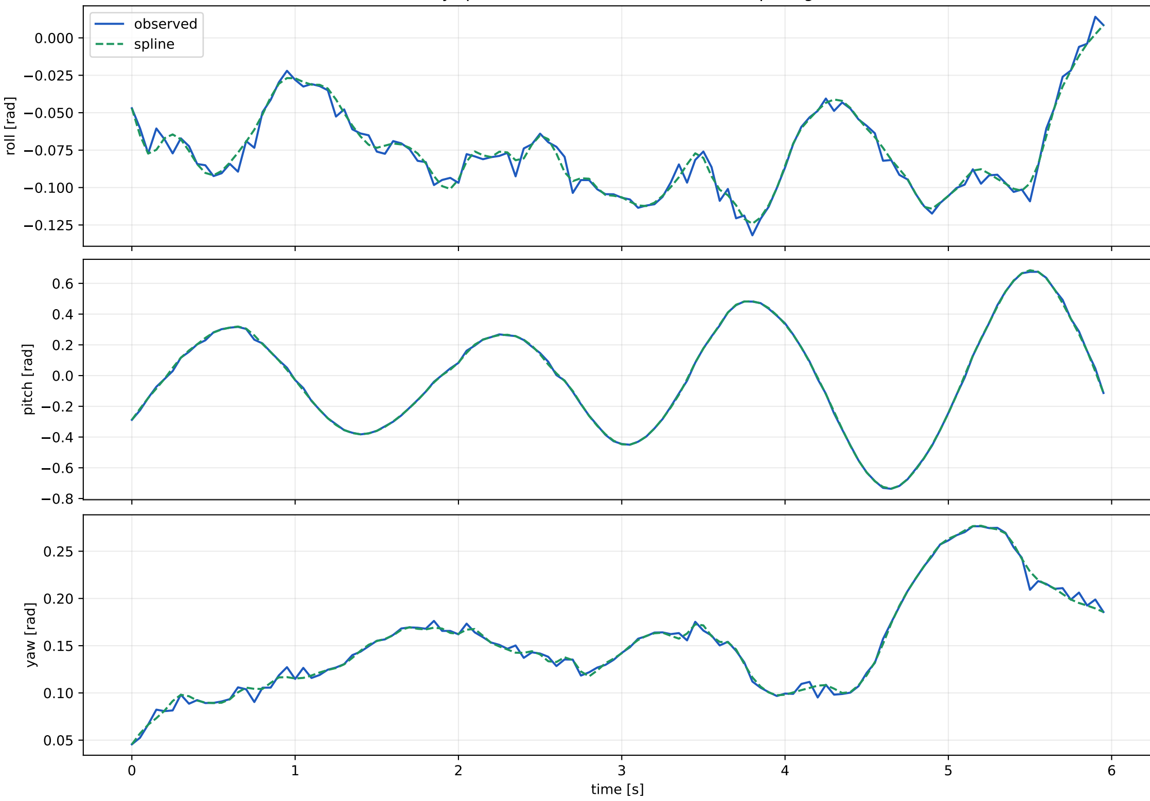
Pose-only spline orientation fit; selected knot spacing=0.1s
