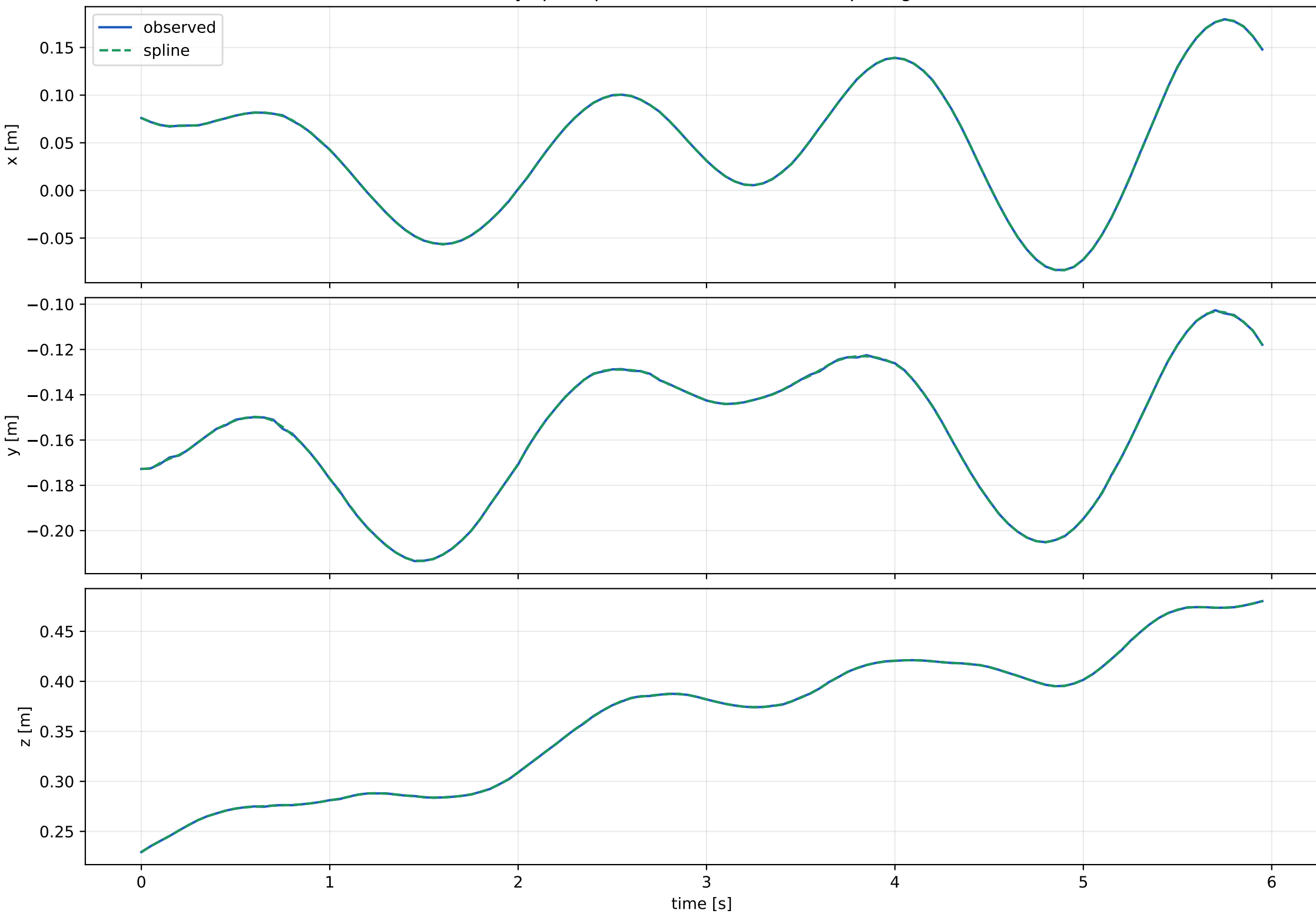
Pose-only spline position fit; selected knot spacing=0.1s
