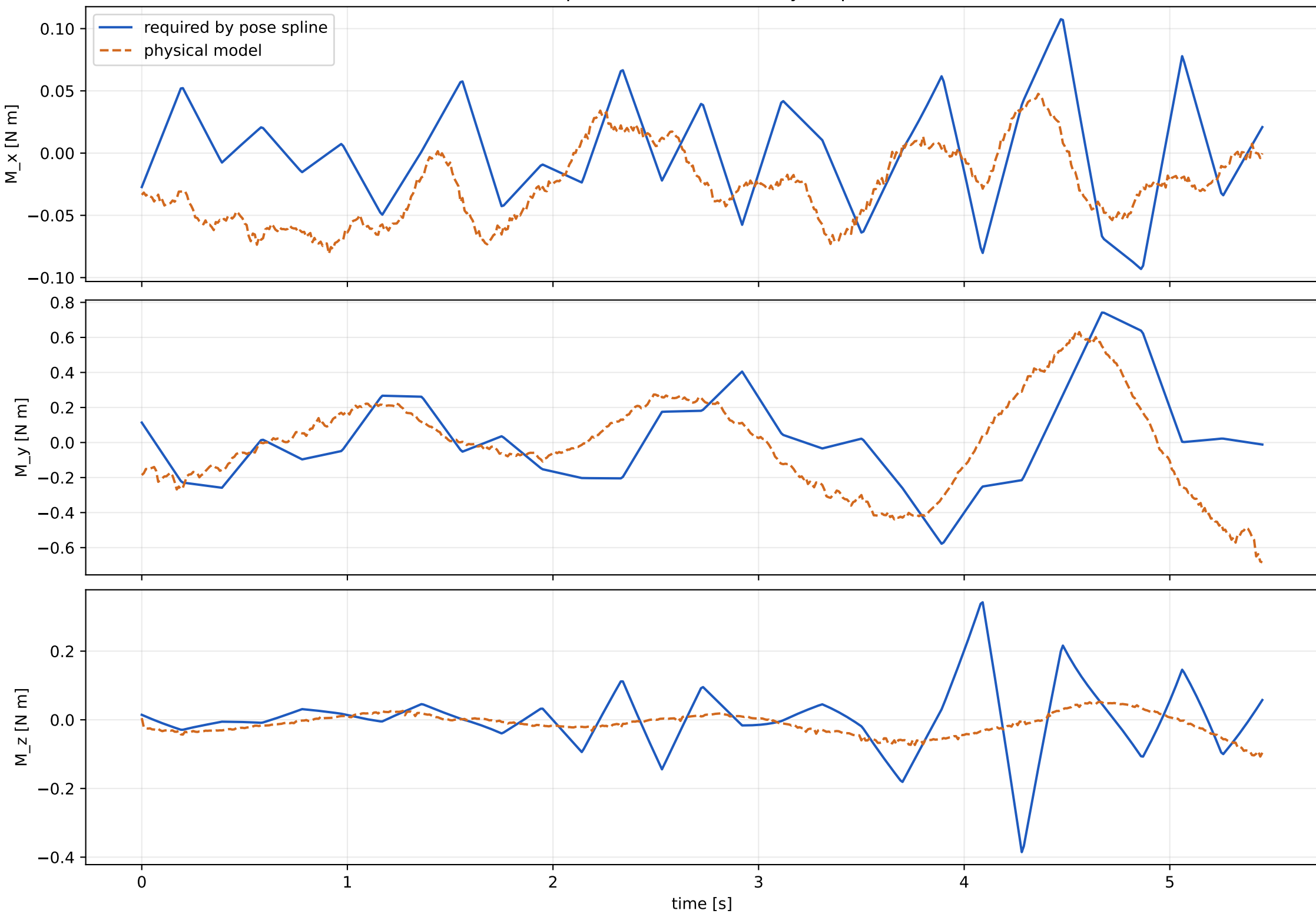
Required and modeled body torque
