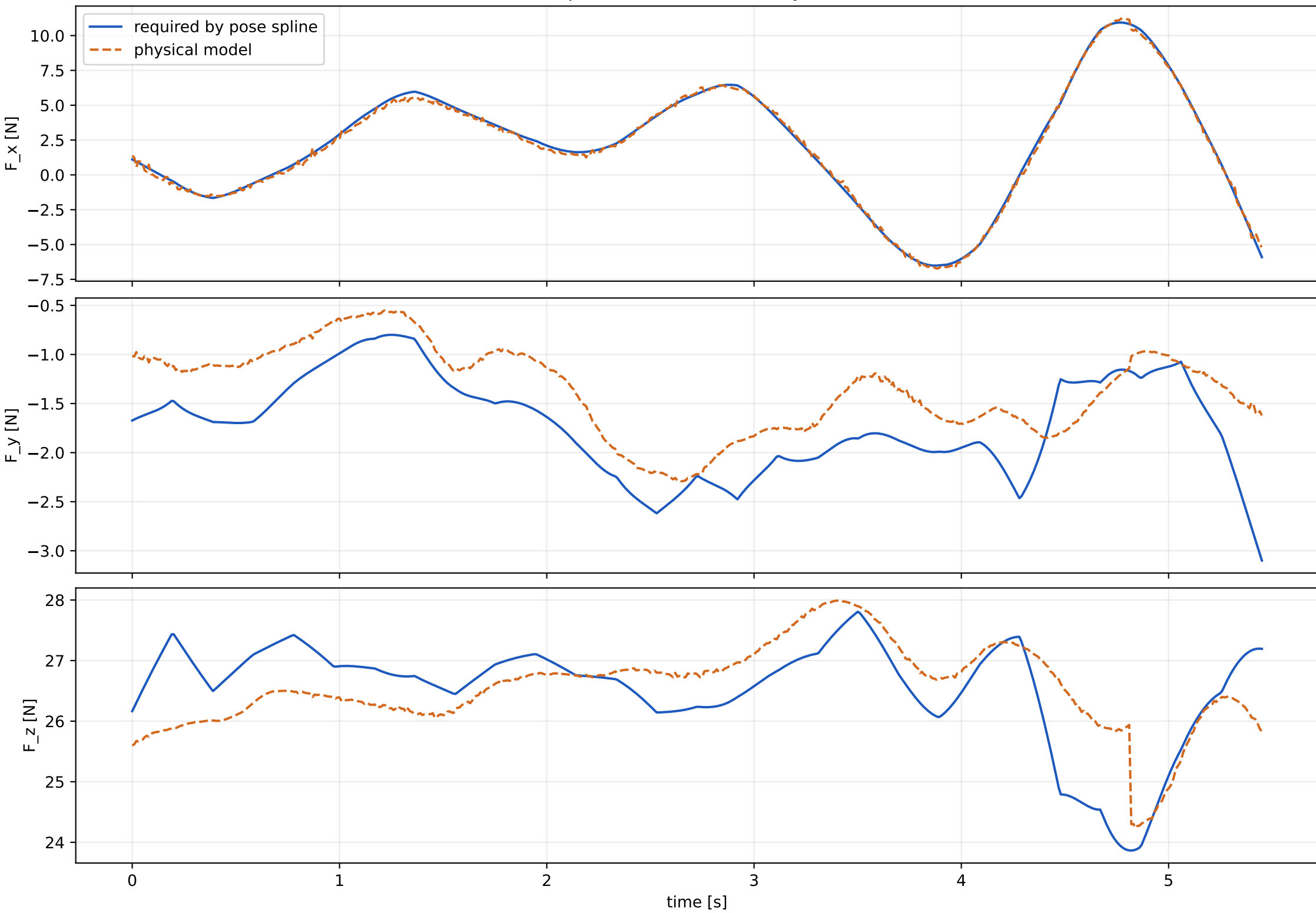
Required and modeled body force
