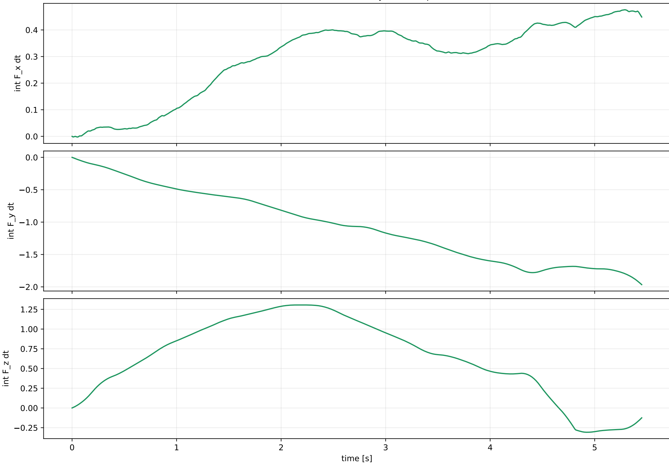
Cumulative residual body force impulse
