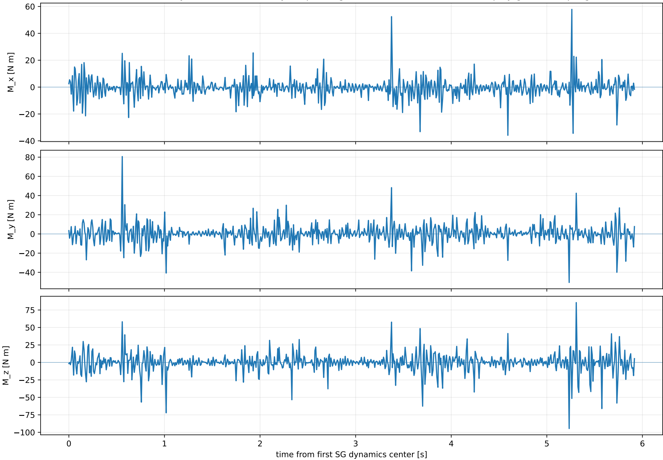
Raw inverse-dynamics residual body torque; degree-5 SG W=0.0528808s ; no replay-grid resampling
