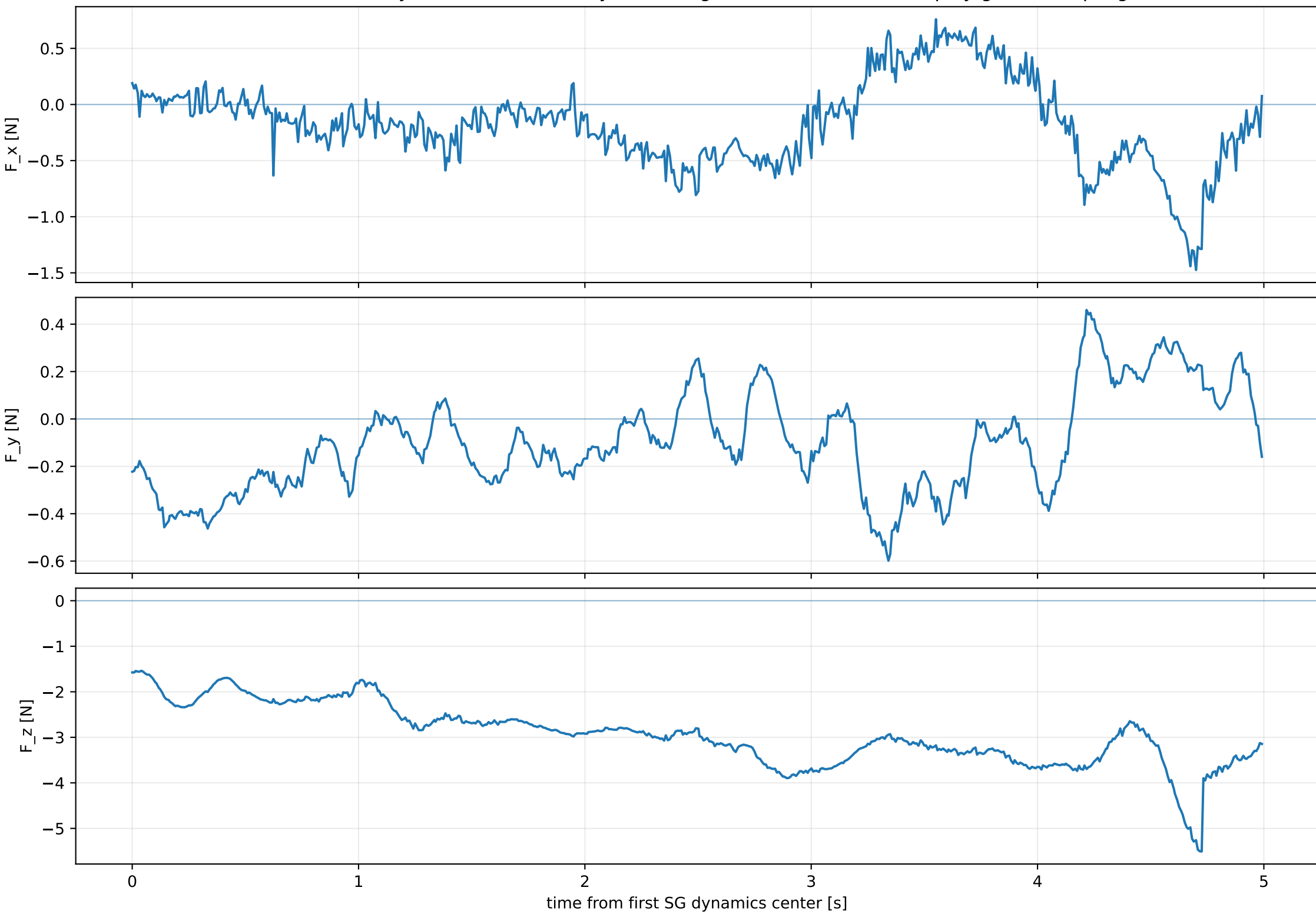
Raw inverse-dynamics residual body force; degree-5 SG W=0.5s; no replay-grid resampling
