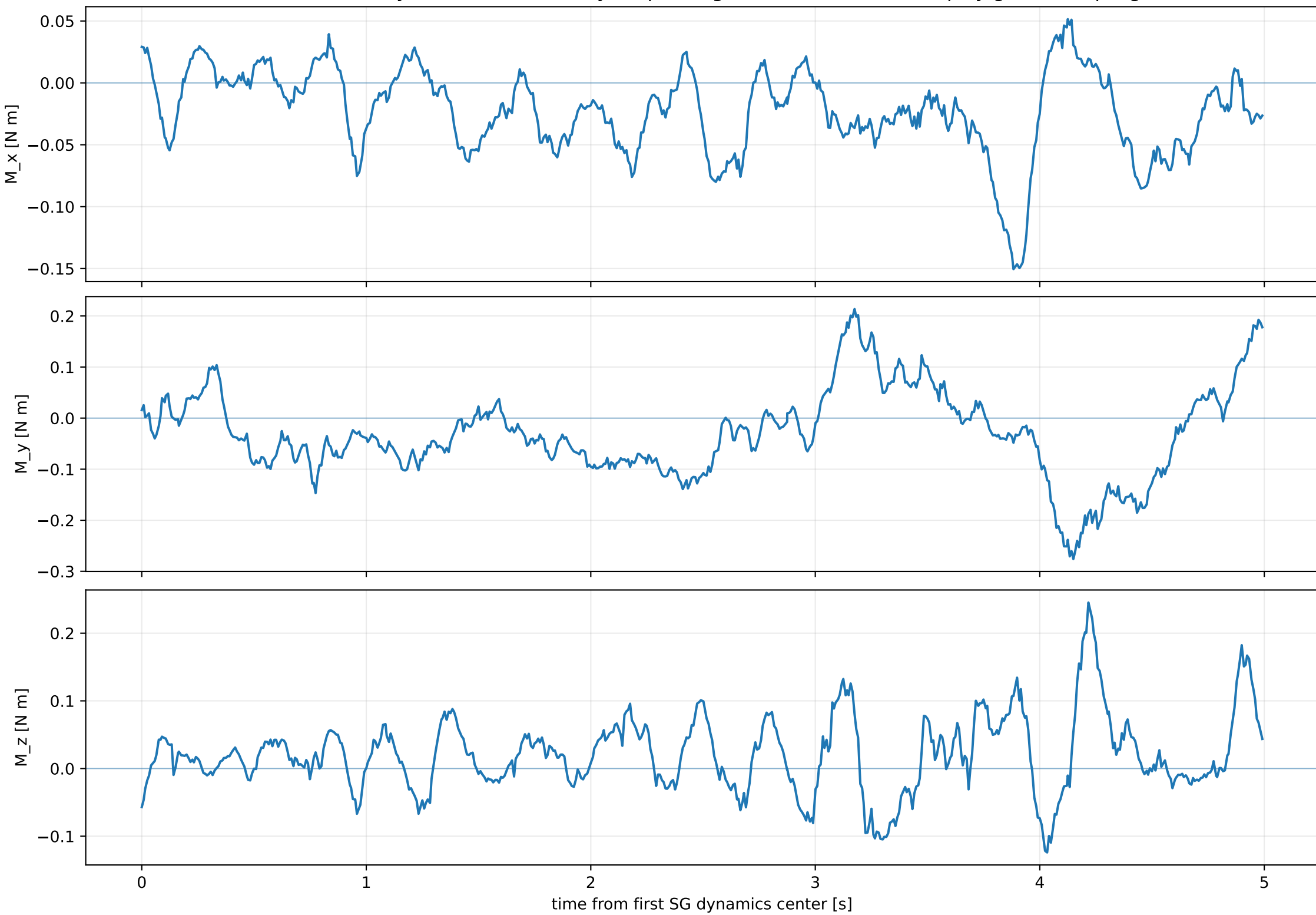
Raw inverse-dynamics residual body torque; degree-5 SG W=0.5s; no replay-grid resampling
