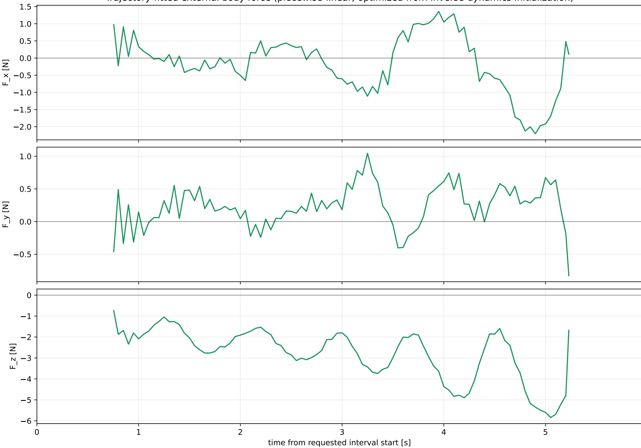
Trajectory-fitted external body force (piecewise-linear; optimized from inverse-dynamics initialization)
