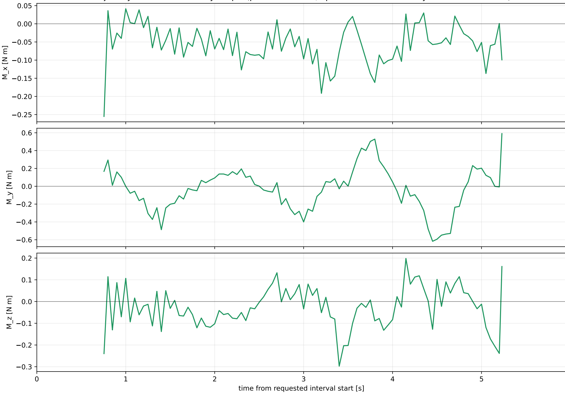
Trajectory-fitted external body torque (piecewise-linear; optimized from inverse-dynamics initialization)
