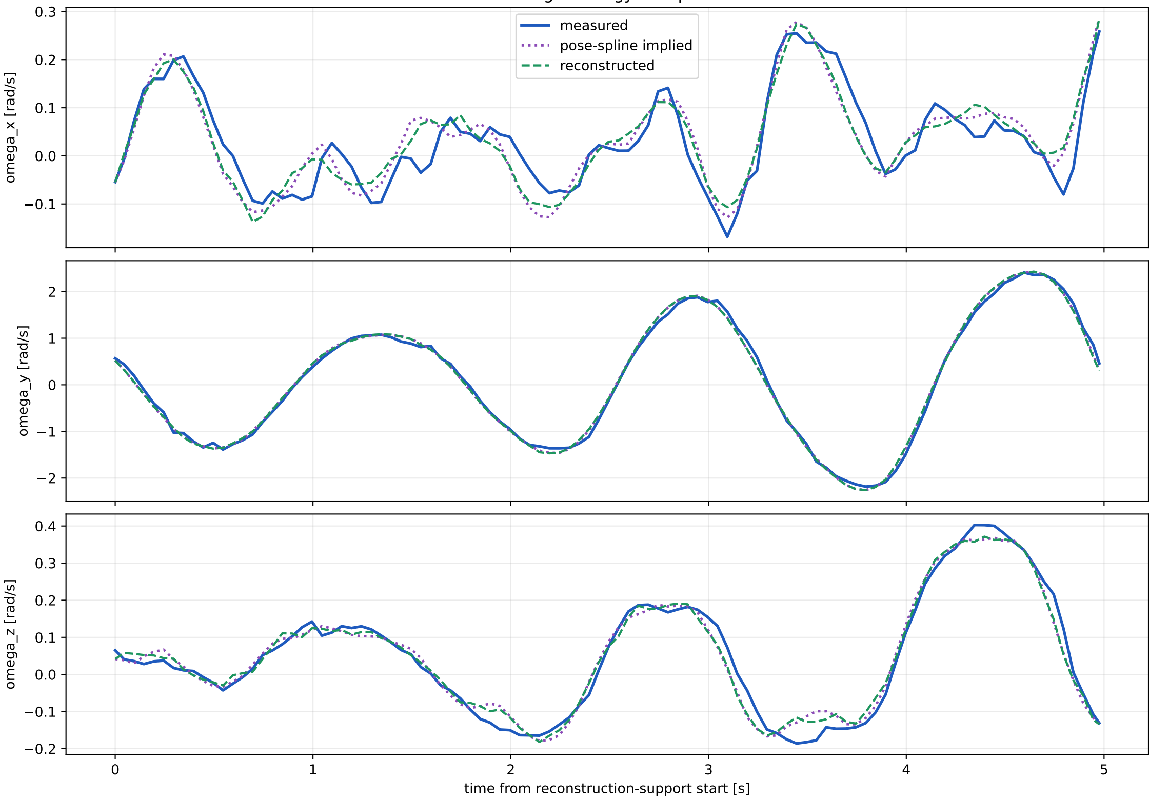
Diagnostic: gyroscope
