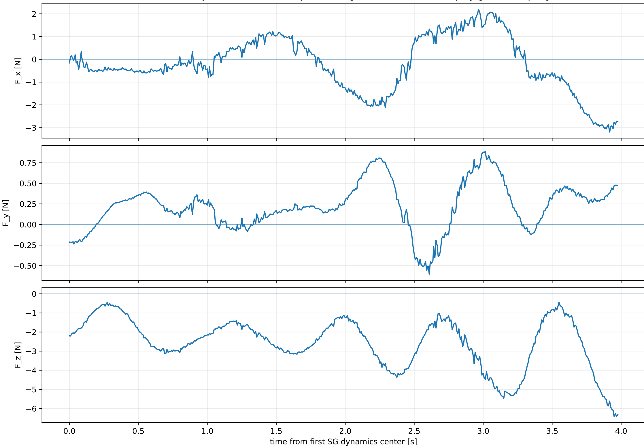
Raw inverse-dynamics residual body force; degree-5 SG W=2s; no replay-grid resampling
