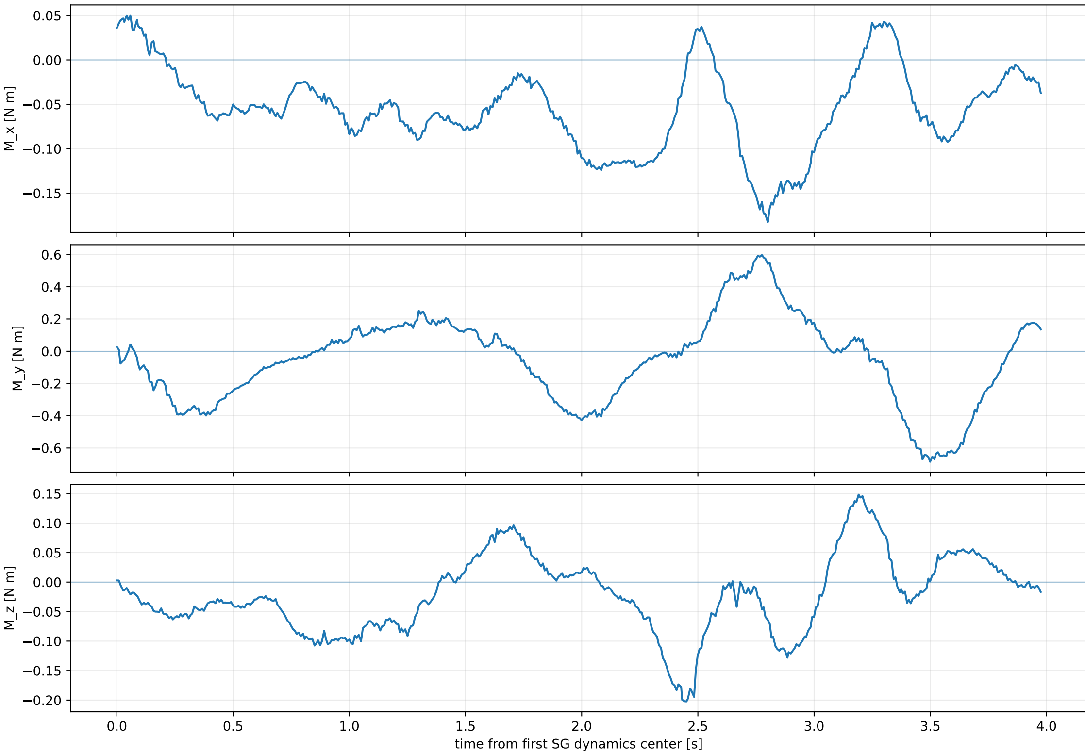
Raw inverse-dynamics residual body torque; degree-5 SG W=2s; no replay-grid resampling
