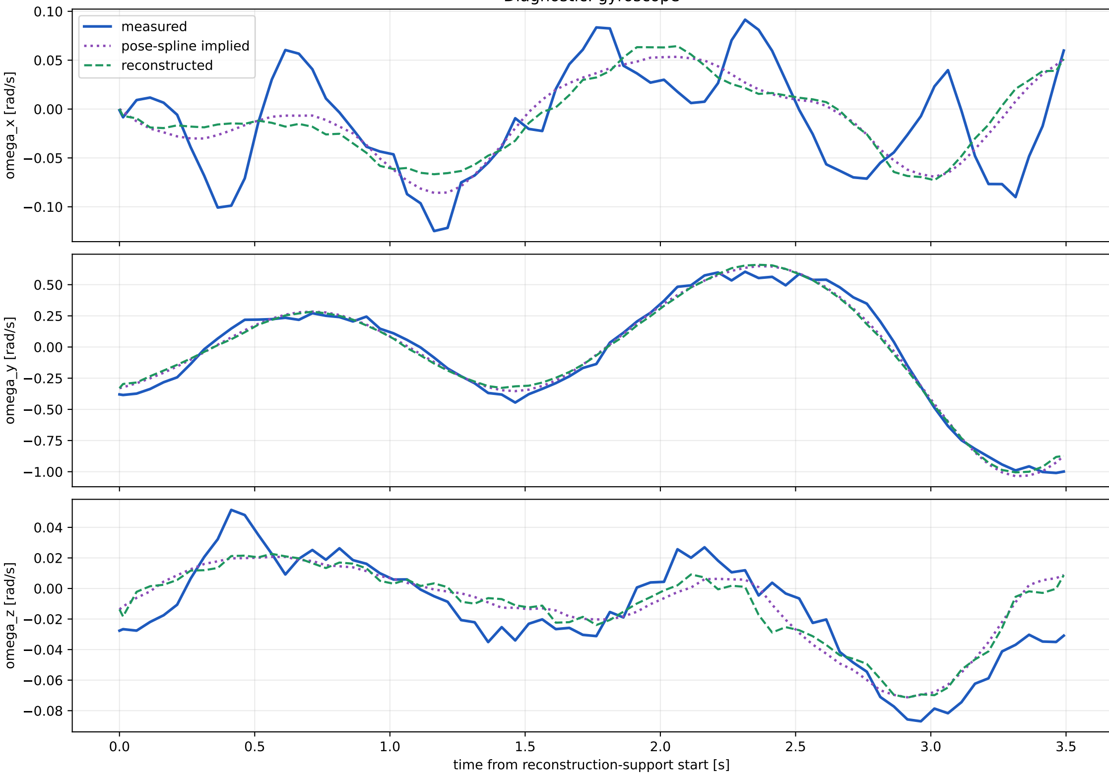
Diagnostic: gyroscope
