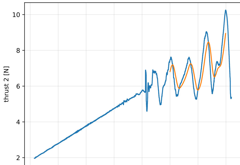
failure1: command and fitted first-order thrust, tau=0.25231 s
