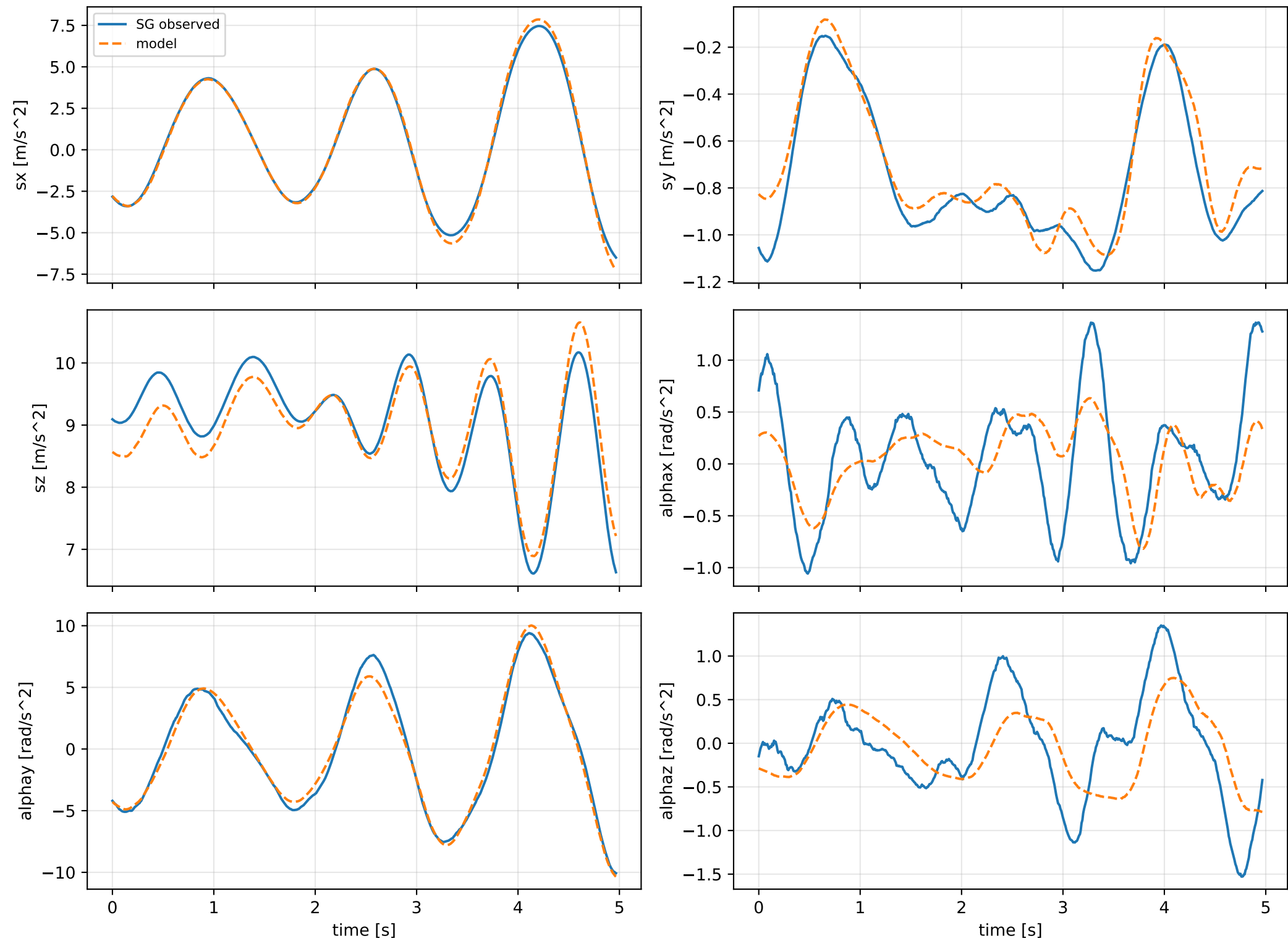
failure1: acceleration objective
