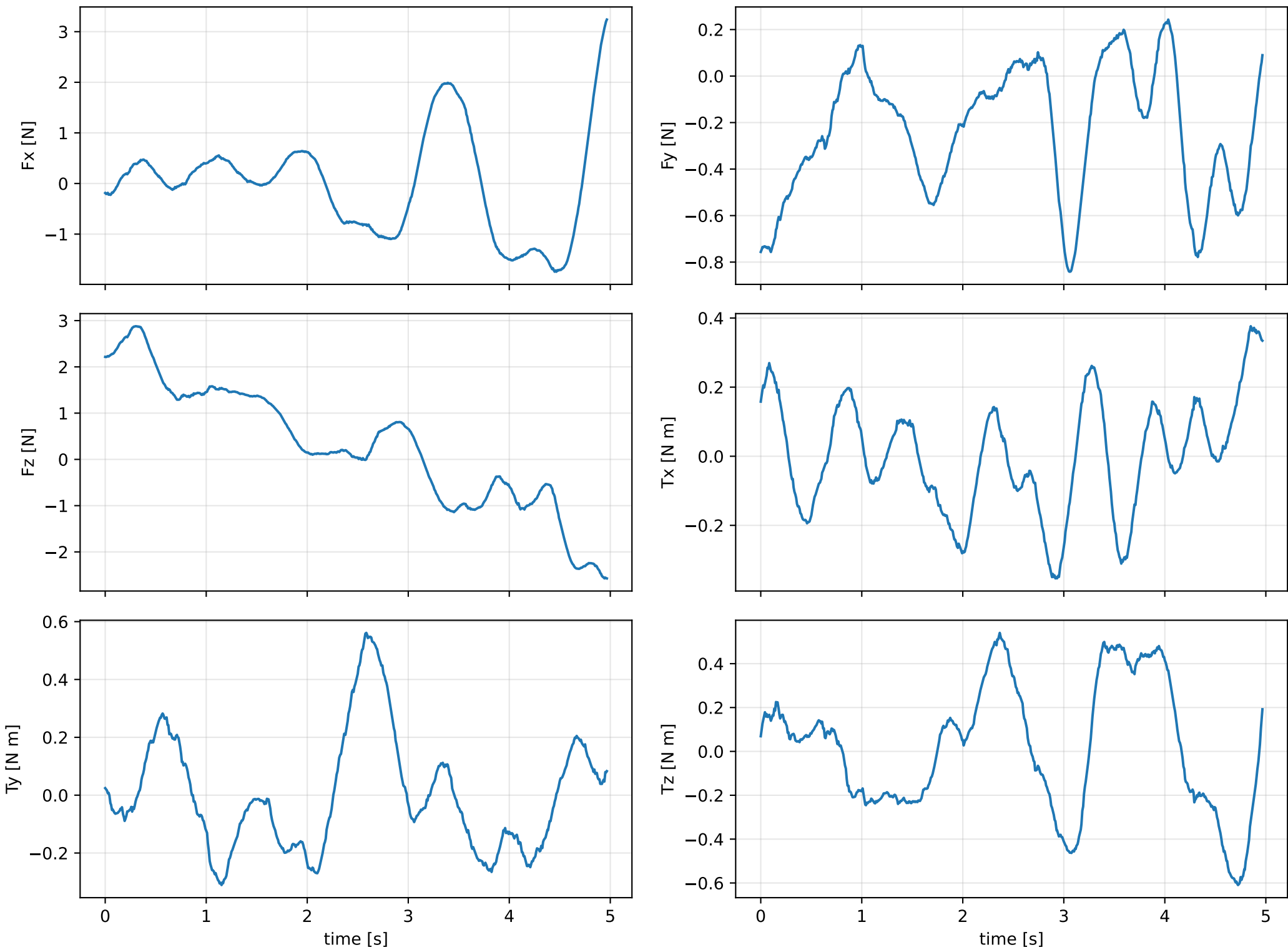
failure1: first-order-model residual wrench
