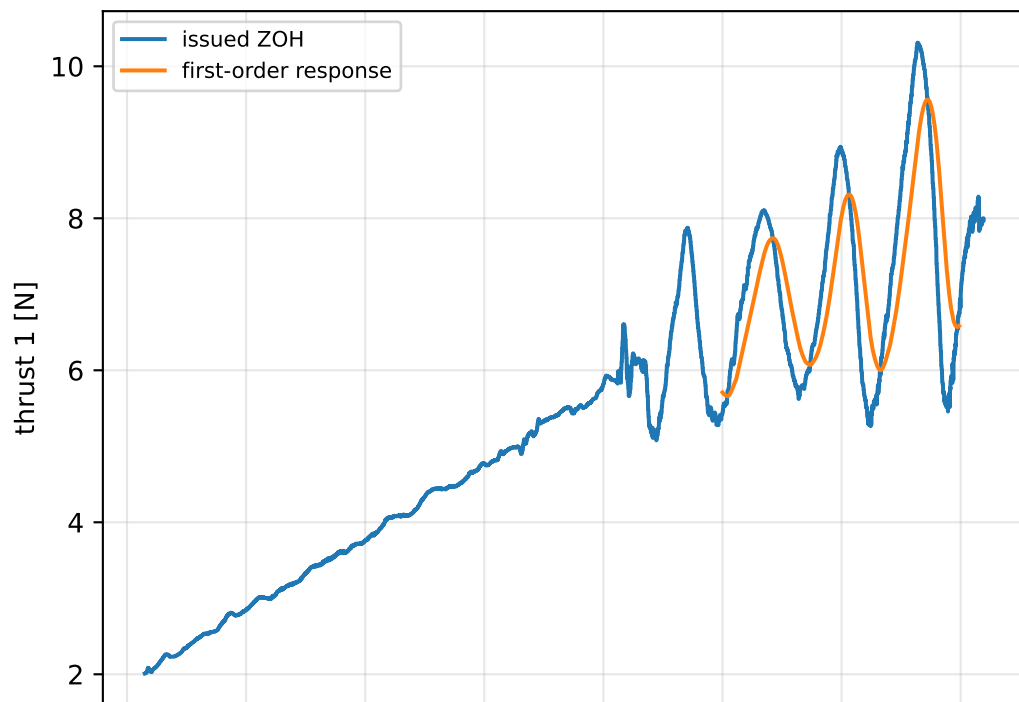
failure1: command and fitted first-order thrust, tau=0.25231 s
