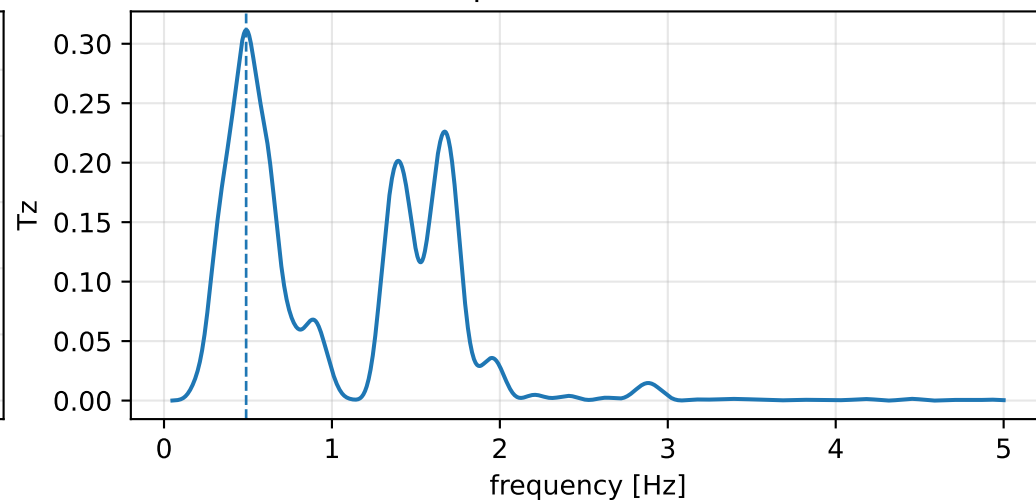
peak 0.489 Hz
