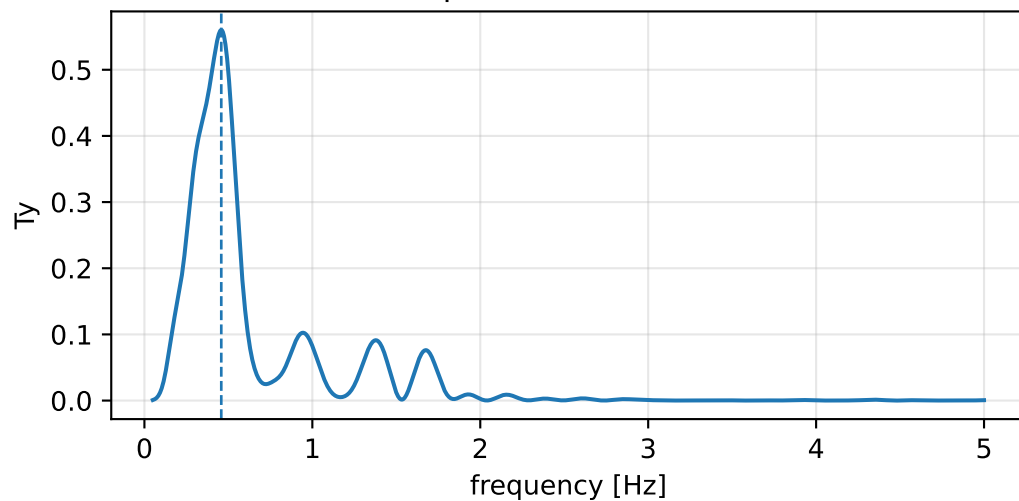
peak 0.4577 Hz
