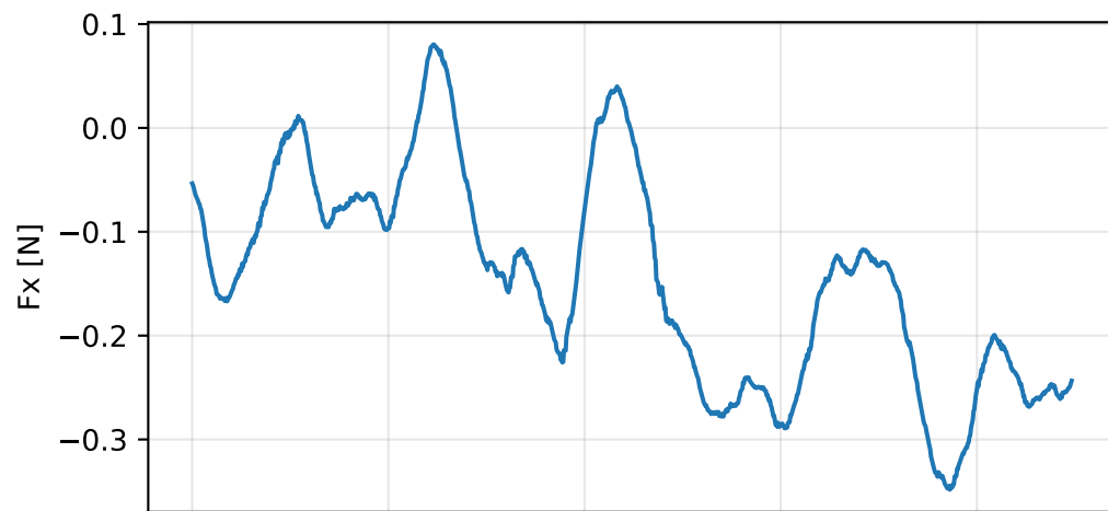
success: first-order-model residual wrench
