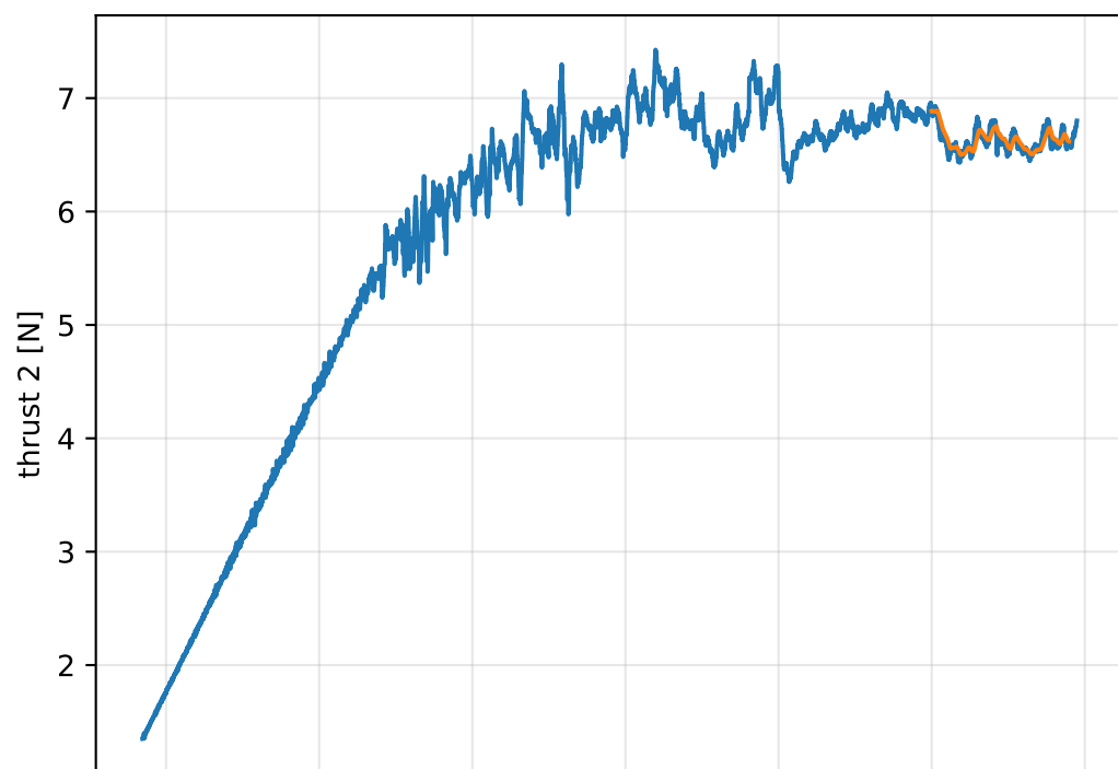
success: command and fitted first-order thrust, tau=0.240612 s
