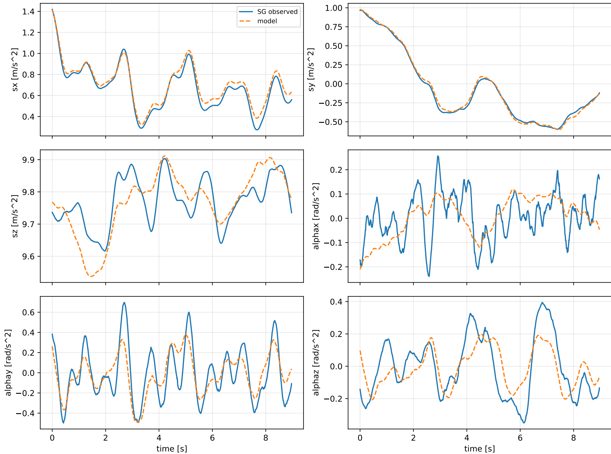
success: acceleration objective
