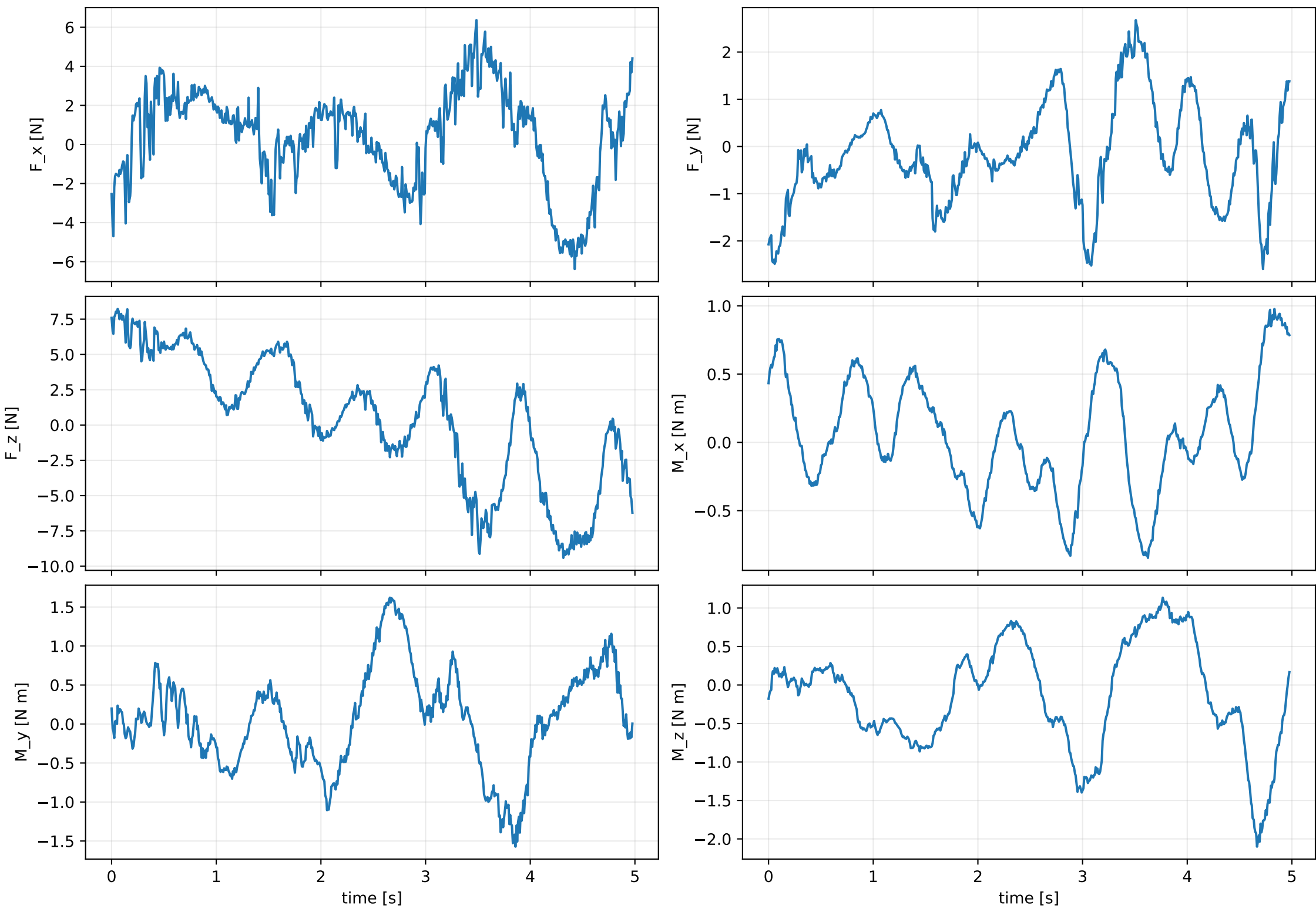
Raw inverse-dynamics residual body wrench
